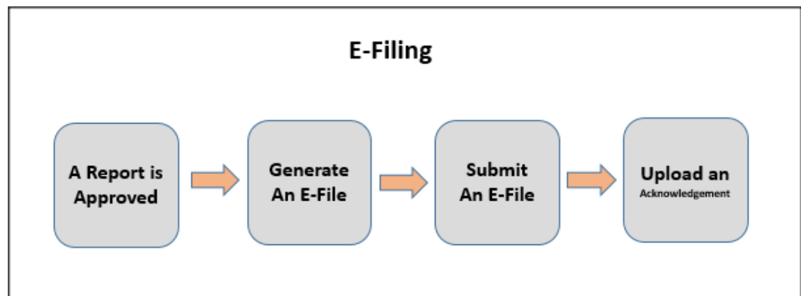
Figure 8-1 E-Filing Workflow
