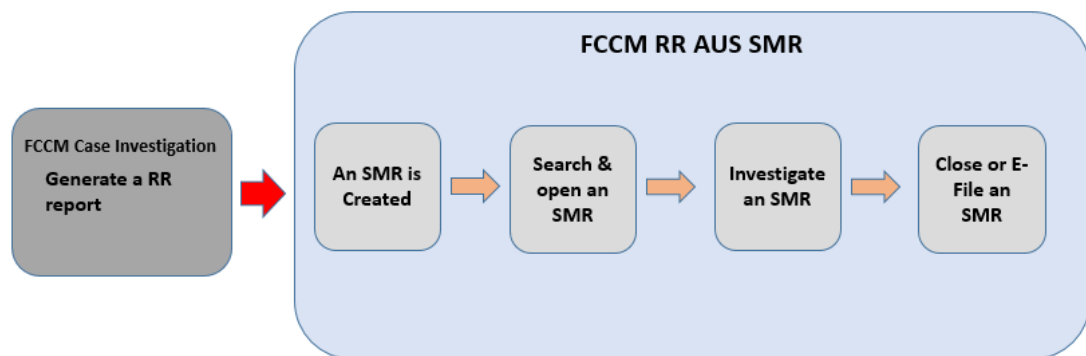
Figure 2-1 Report Workflow
