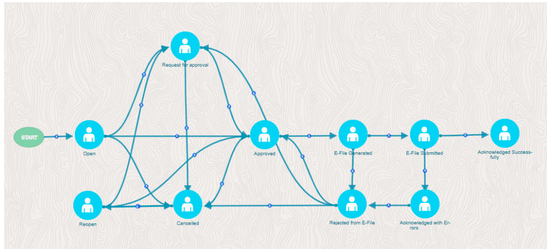
Figure 2-2 User Workflow
