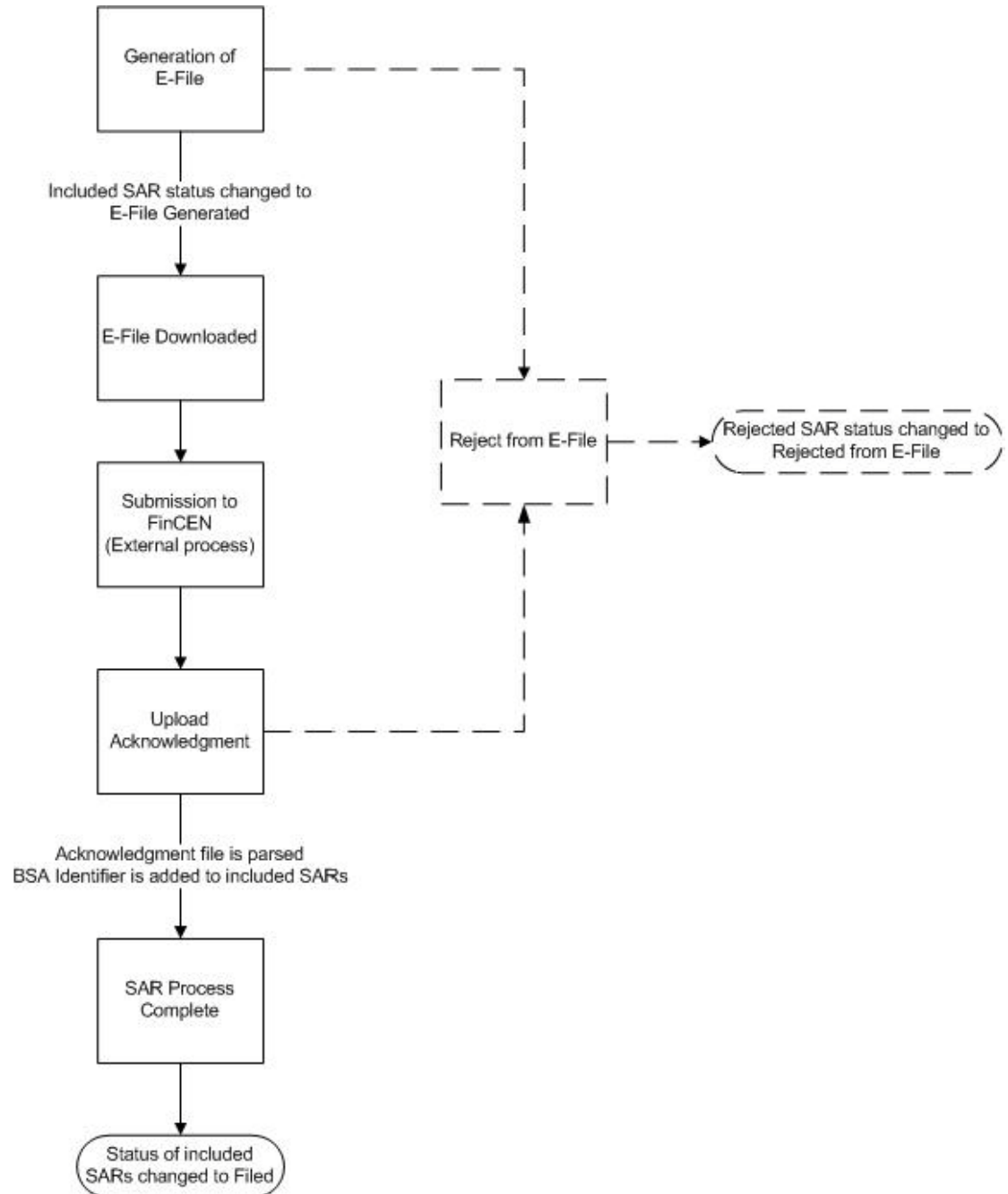
Figure 8-1 Workflow for Filing the Regulatory Report
