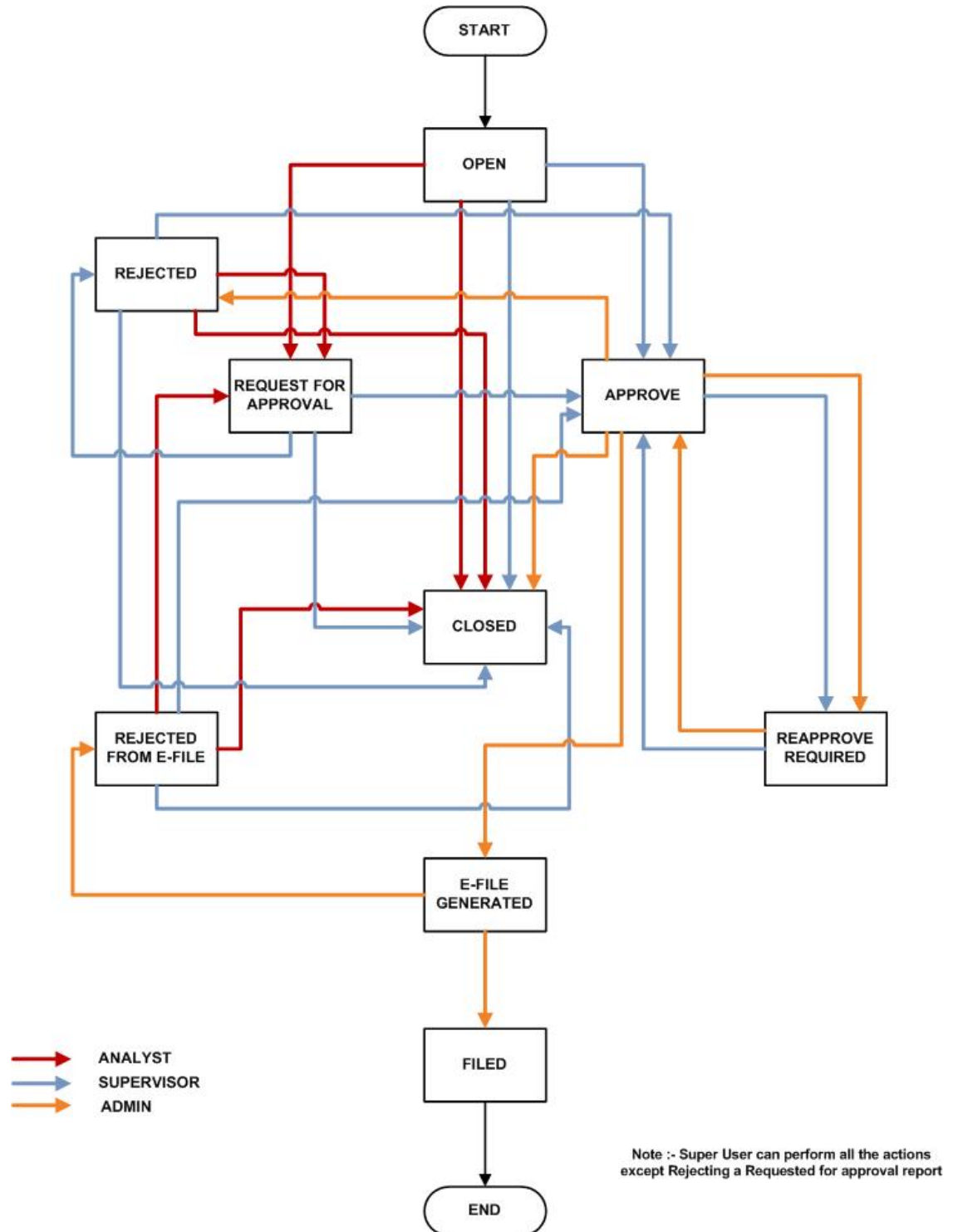
Figure 2-1 OFS CRR CS USSAR Cloud Service Workflow
