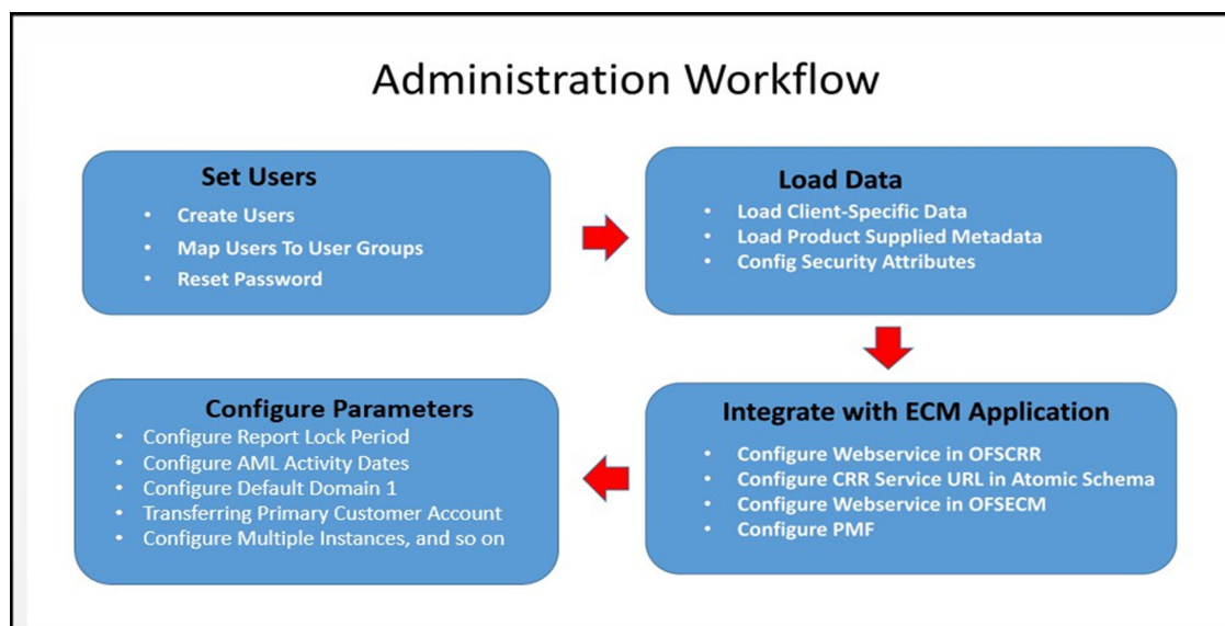
Figure 2-1 Administrator workflow
