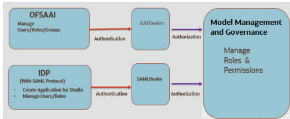
Figure 6-2 Authentication and Authorization process in STSA
