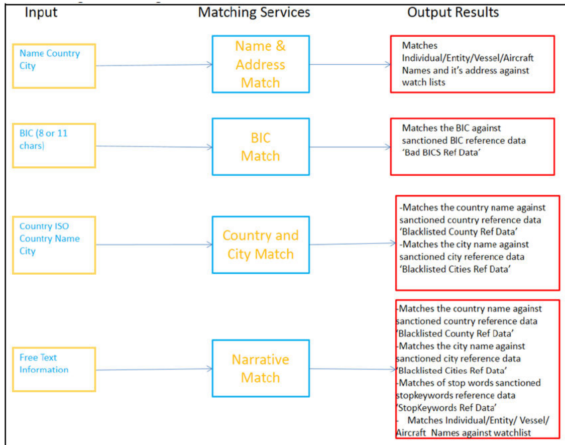
Figure 4-1 Matching Webservices
