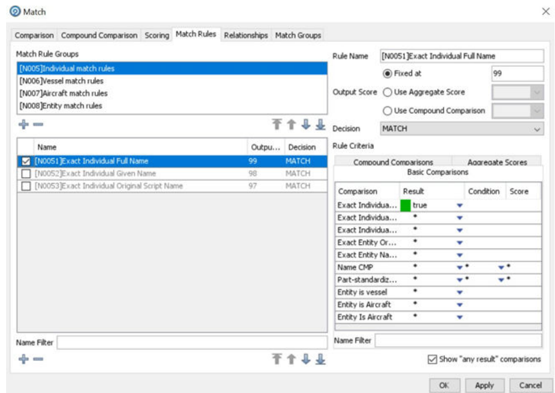
Figure 9-3 Match Window
