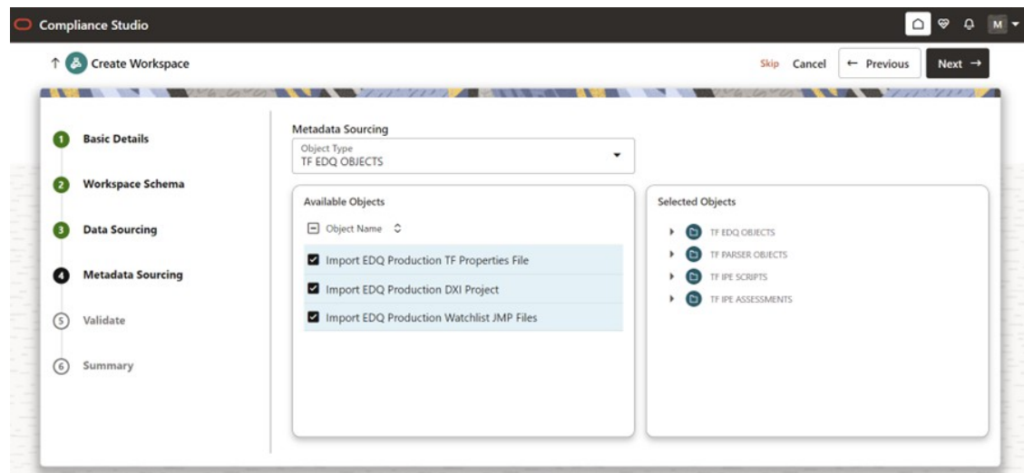
Figure 12-11 Metadata Sourcing
