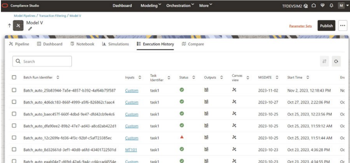
Figure 12-28 Execution History
