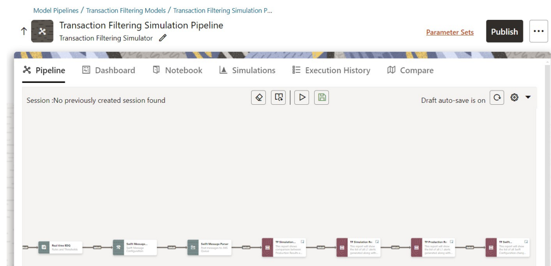
Figure 12-22 Pipeline Canvas
