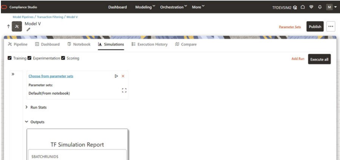
Figure 12-27 Simulation Tab
