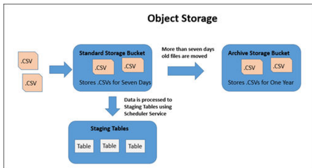
Figure 3-1 Object Storage
