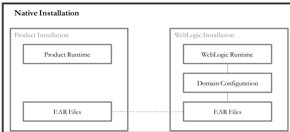
Figure 4: Native Architectures
