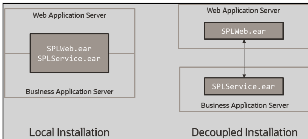
Figure 21: Installation Modes
