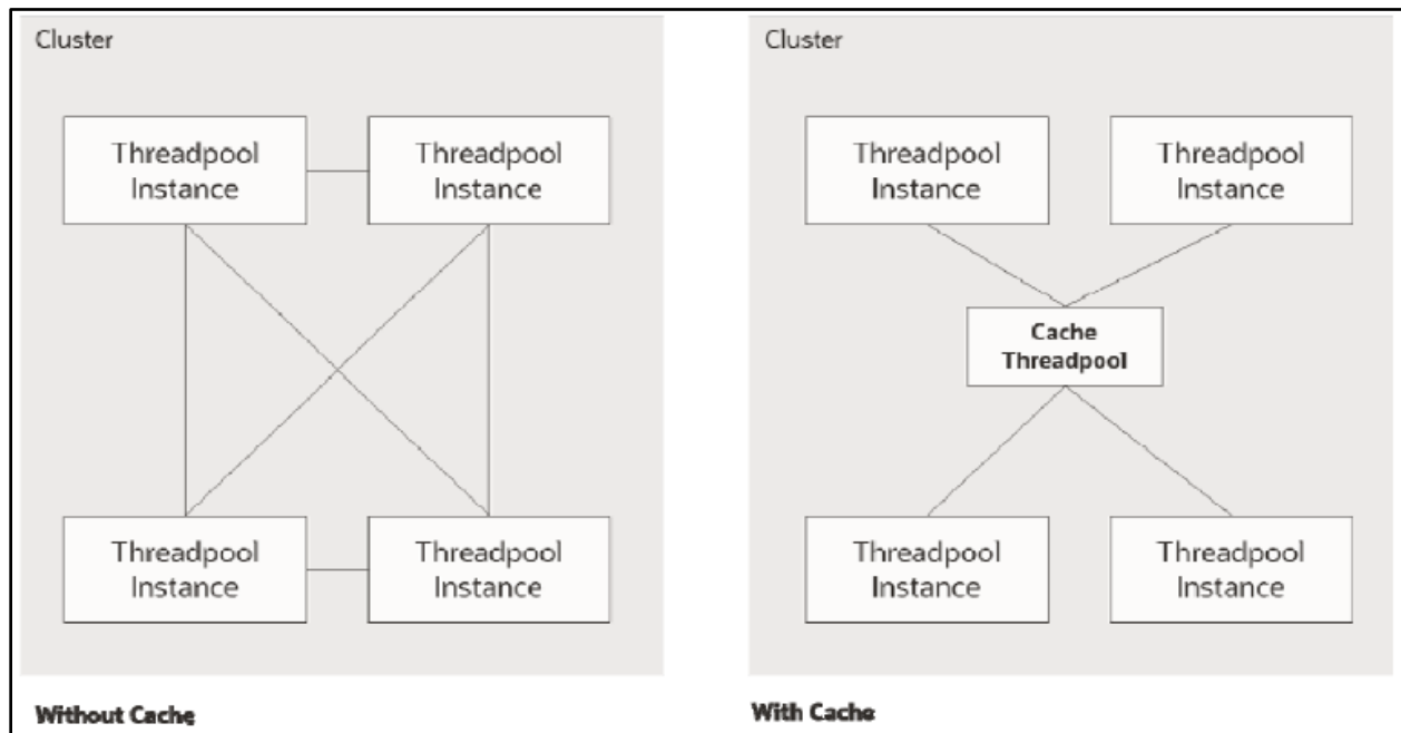
Figure 33: Cache Architecture
