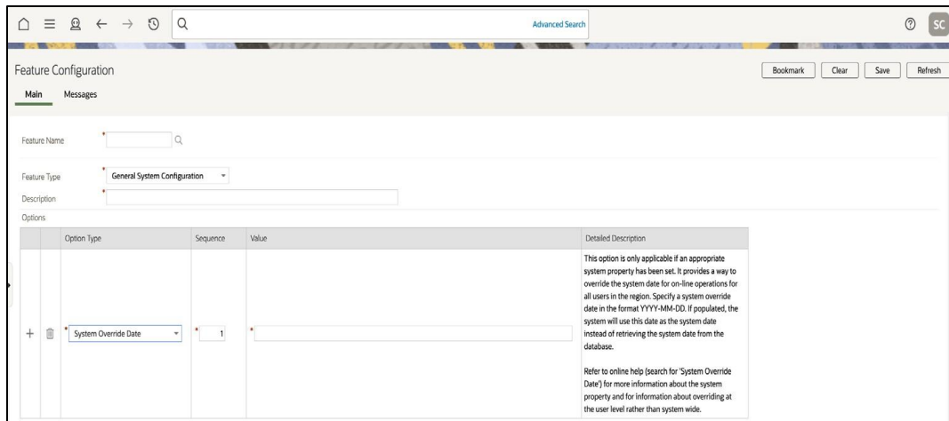
Figure 39: Feature Configuration
