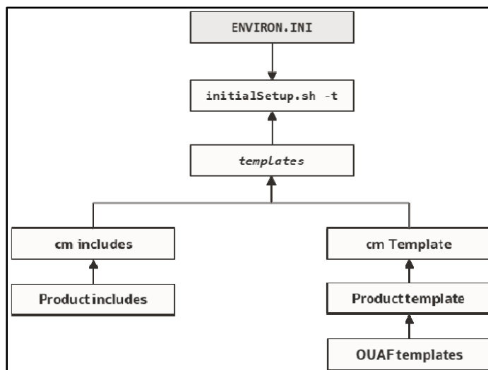
Figure 37: Template Hierarchy
