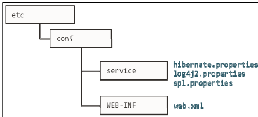
Figure 23: Business Application Server Configuration Files
