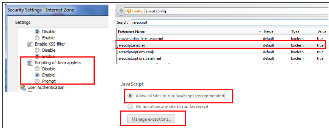
Figure 17: Javascript Settings
