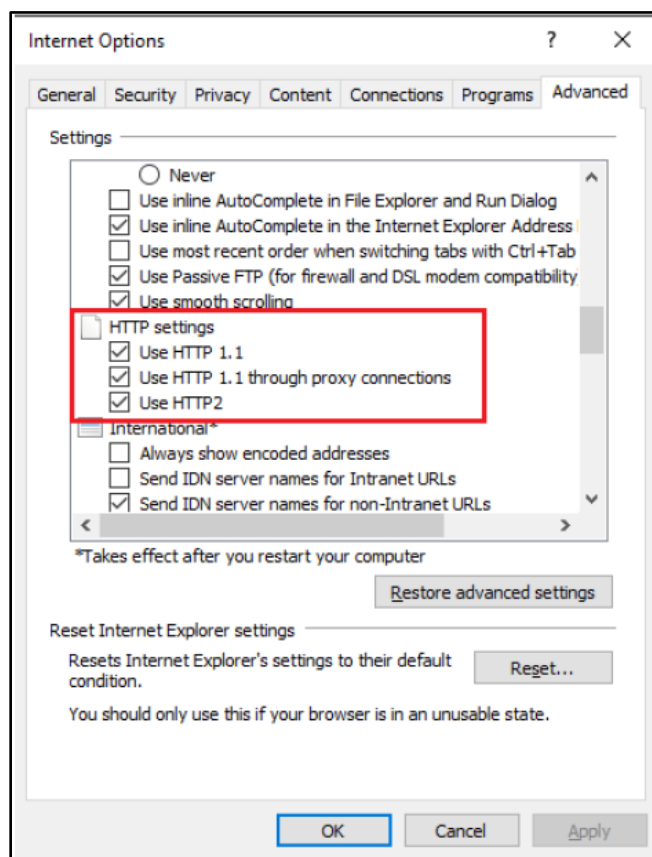
Figure 16: HTTP 1.1 Settings
