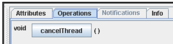
Figure 43: CancelThread Example
