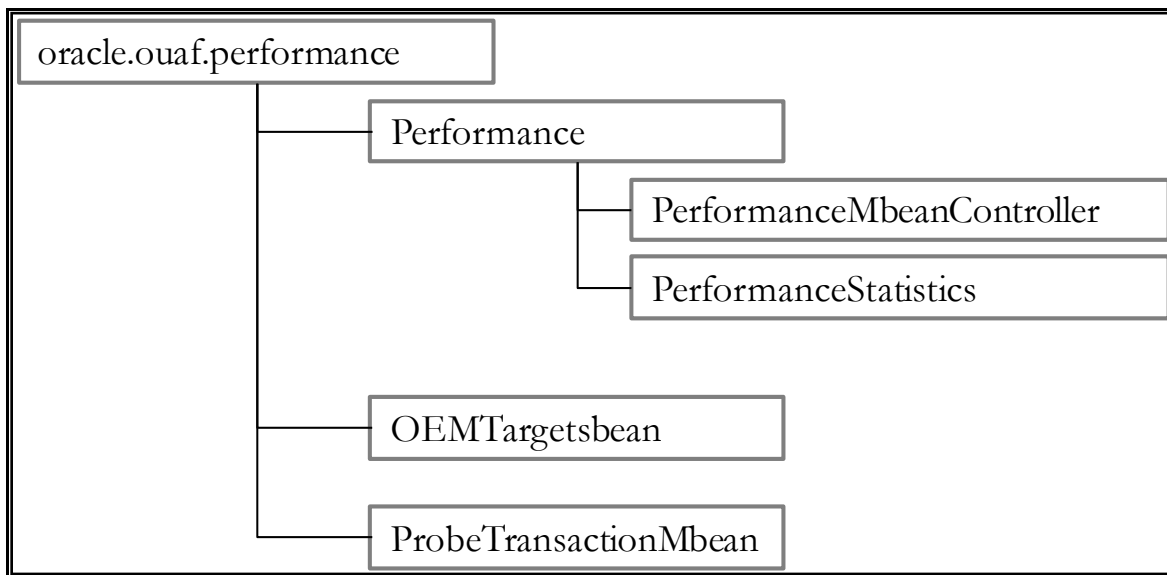
Figure 12: Business Application Server Mbeans
