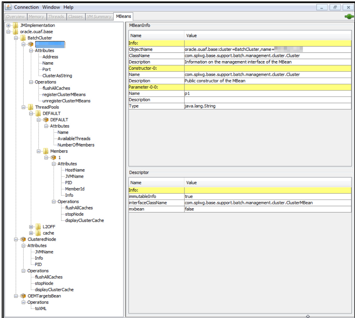
Figure 13: Batch Server Mbeans in jconsole Example
