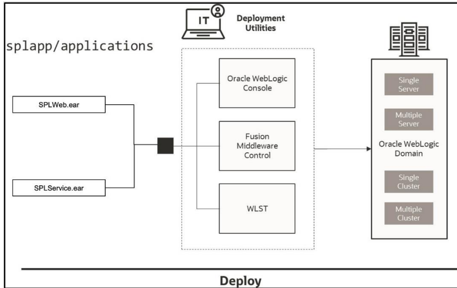
Figure 20: Web Application Server Deployment Process
