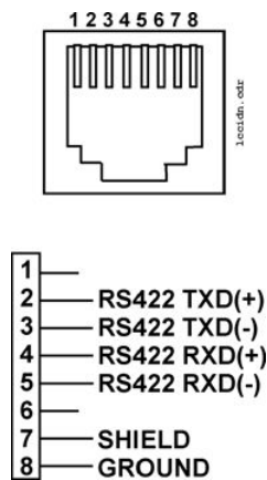
Figure 10-1 RS422 Mode
