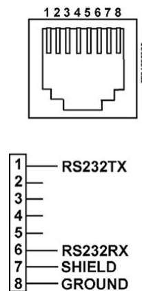
Figure 10-2 RS232 Mode
