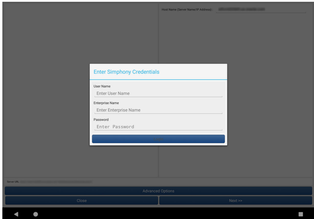
Figure 8-3 Symphony Credentials
