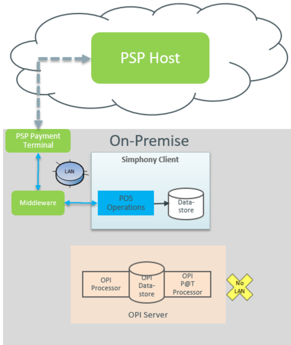
Figure 13-5 Middleware Mode Architecture With or Without Attached PED
