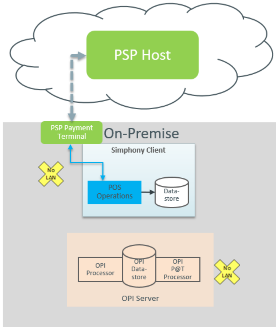
Figure 13-2 Terminal Mode Architecture With Attached PED
