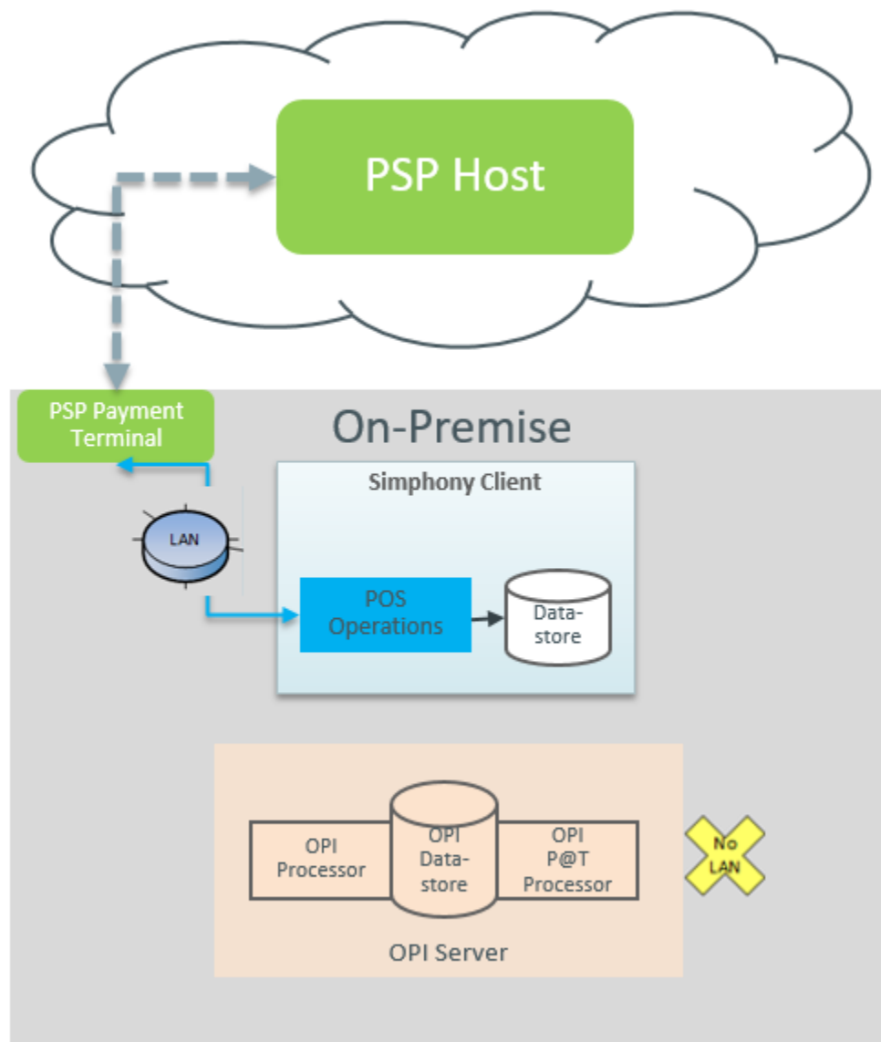
Figure 13-4 Terminal Mode Architecture Without Attached PED
