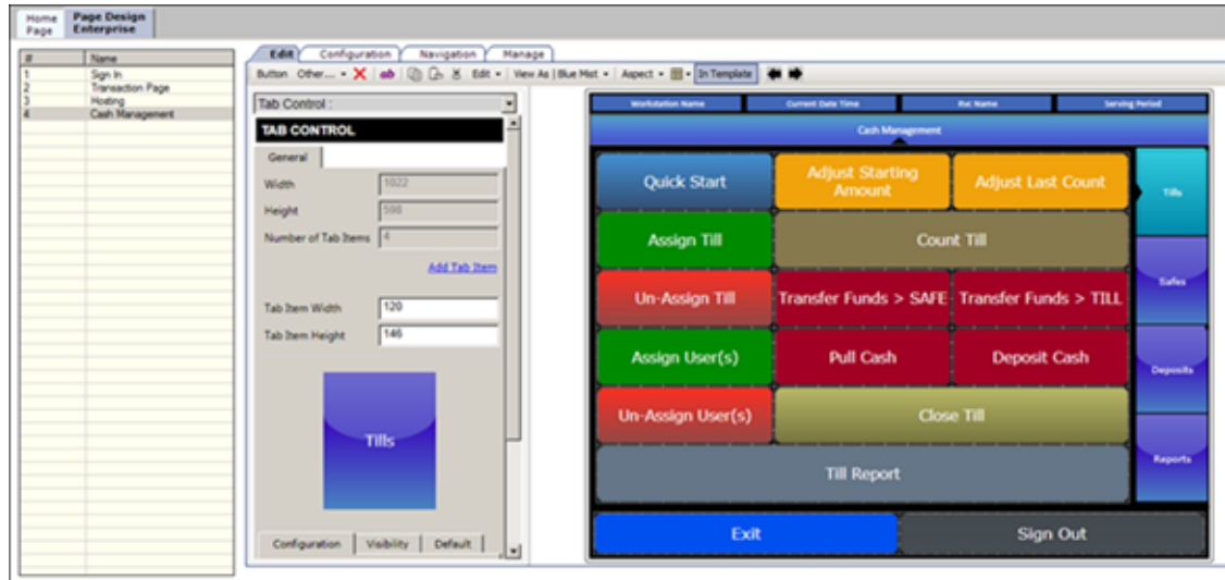
Figure 44-2 Cash Management Touchscreen in Page Design
