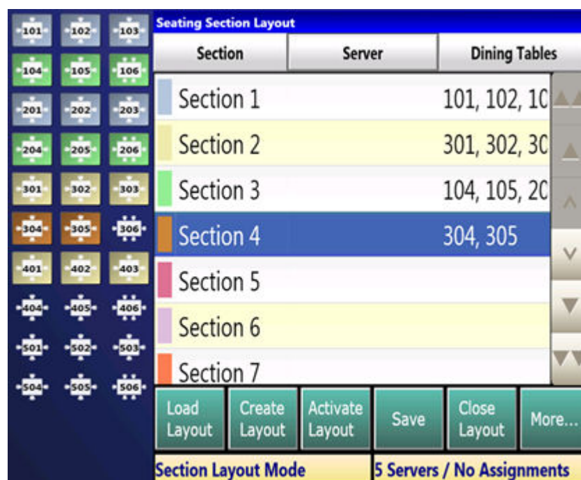
Figure 43-3 Section Layout
