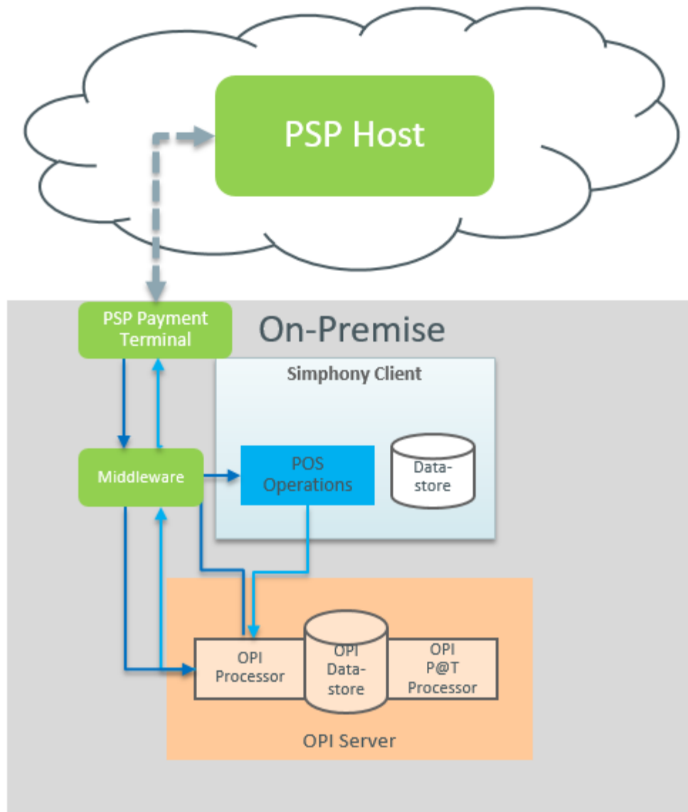
Figure 11-7 Middleware Mode Architecture
