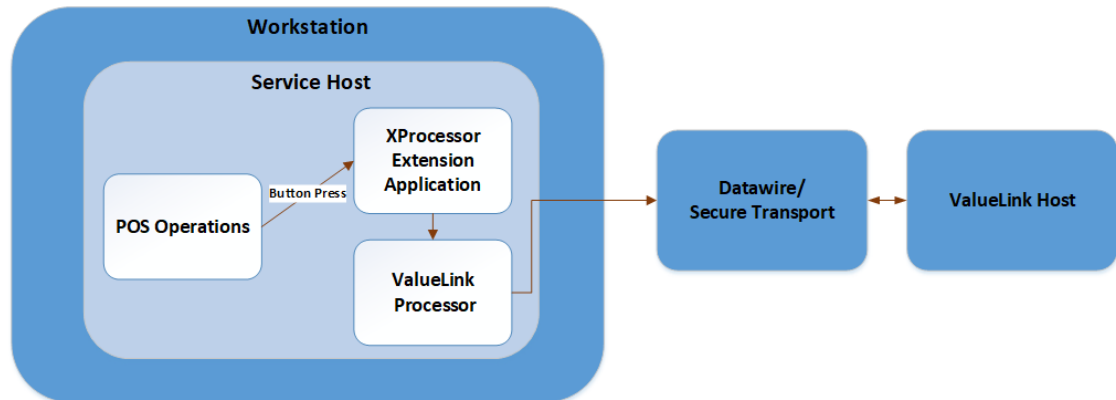
Figure 41-15 ValueLink Processor Data Flow
