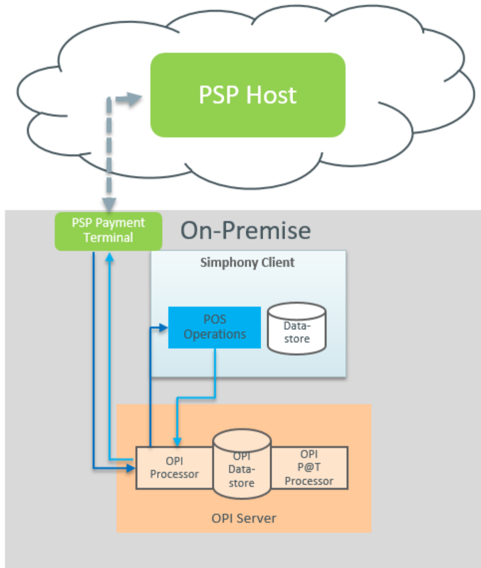
Figure 11-6 Terminal Mode Architecture
