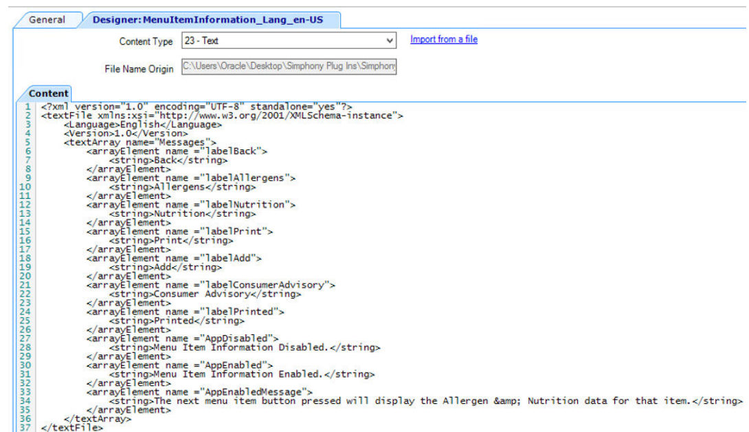
Figure 17-29 Content Area
