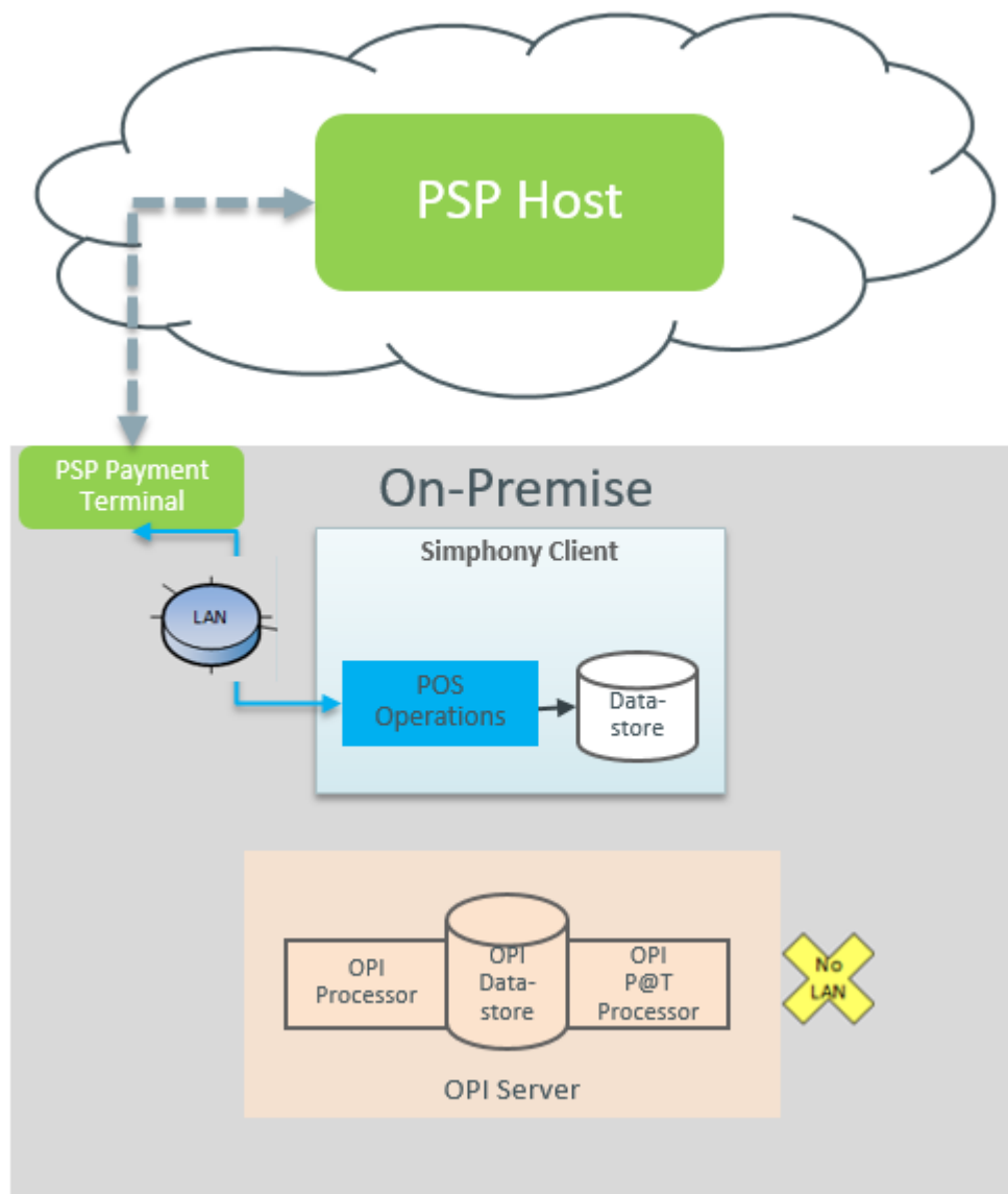
Figure 11-4 Terminal Mode Architecture Without Attached PED
