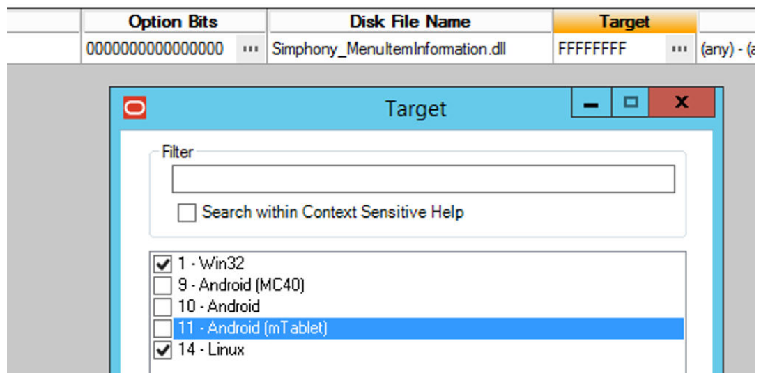
Figure 17-28 Target Dialog
