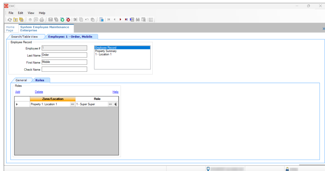
Figure 3-21 Roles Subtab
