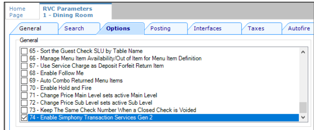
Figure 14-81 RVC Parameters Options
