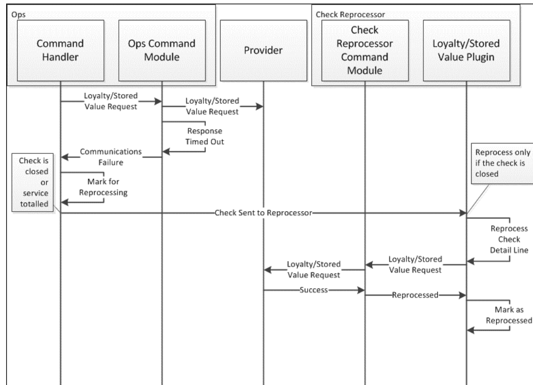
Figure 2-1 - Logic Flow
