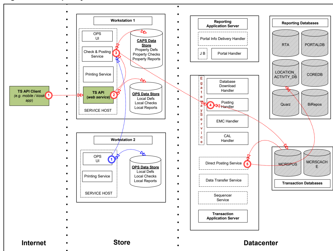
Figure 1-1 - Simphony Architecture
