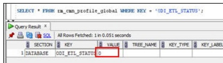
Figure 7-6 Select Statement 1 to Verify Successful Execution
