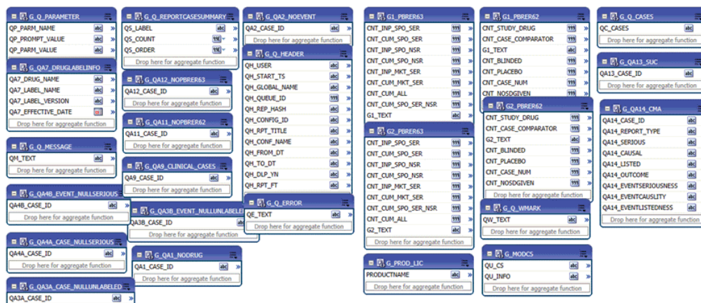
Figure 5-1 Data Sets
