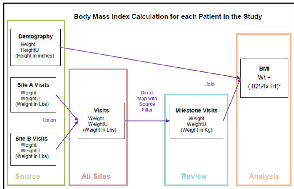
Figure 4-1 Transformation Example: BMI Calculation
