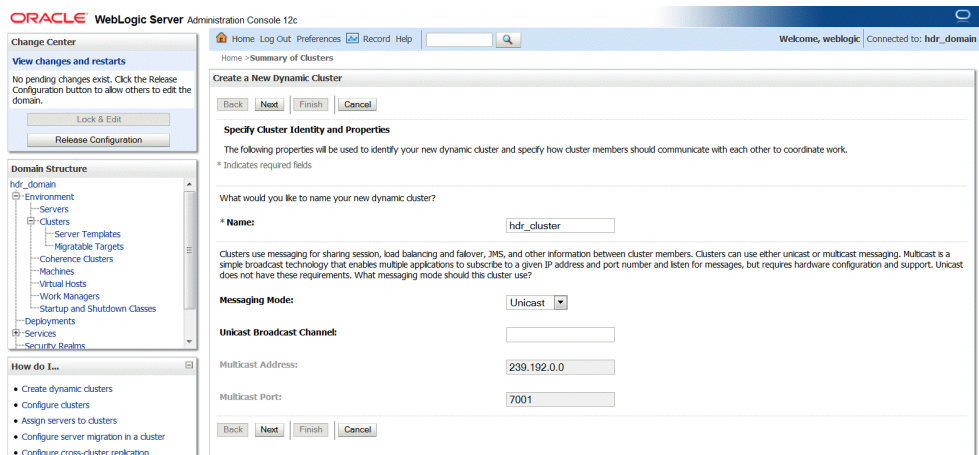
Figure 5-2 Create a New Dynamic Cluster
