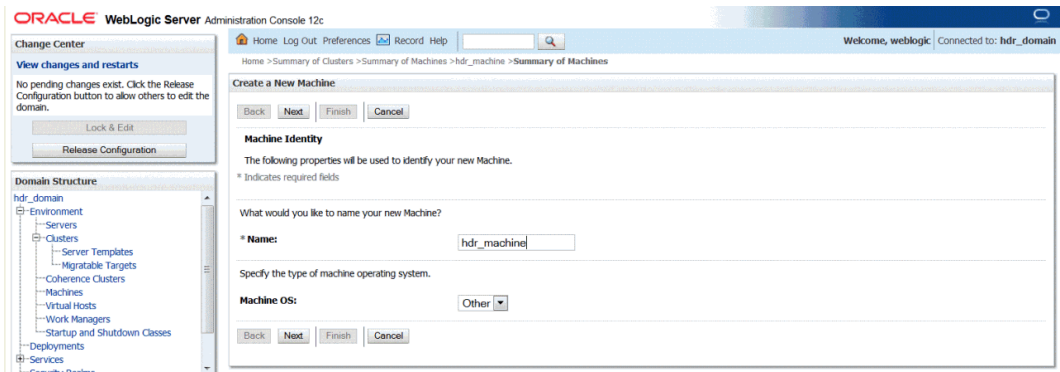
Figure 5-1 Create a New Machine
