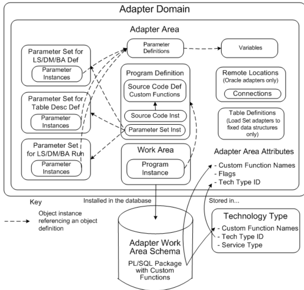
Figure 1-1 Adapter Components and Their Relationships
