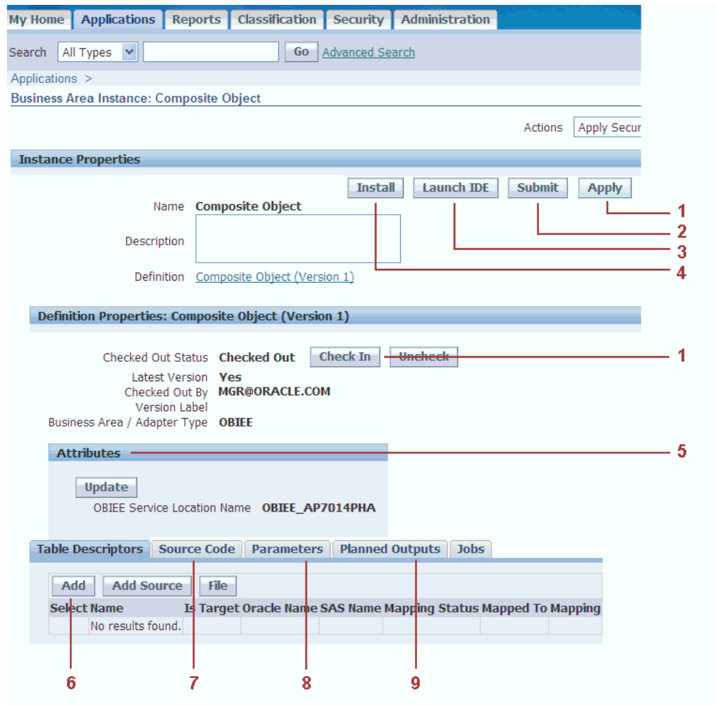
Figure 1-3 Object Properties User Interface
