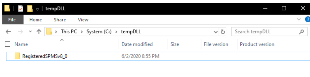
Figure 6-7 RegisteredSPMSv8_0 Folder
