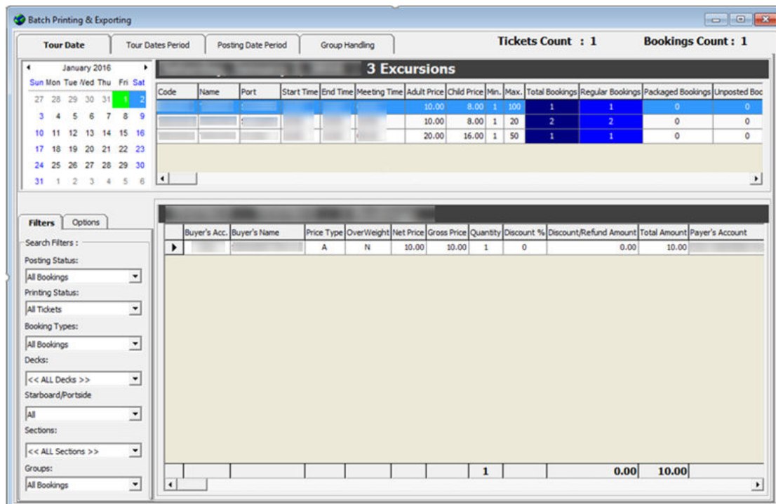
Figure 4-6 Batch Ticket Printing and Exporting
