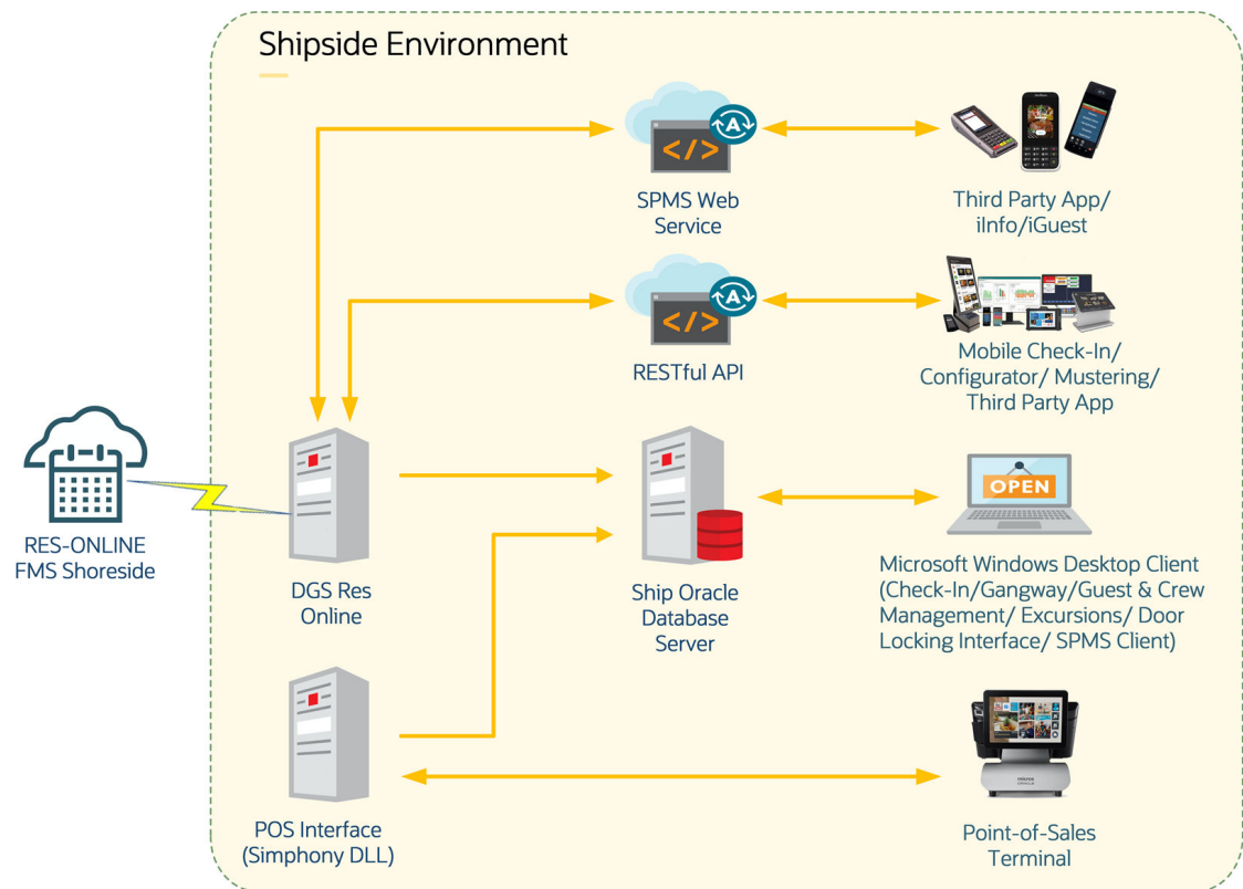
Figure 2-1 SPMS Network Architecture Diagram
