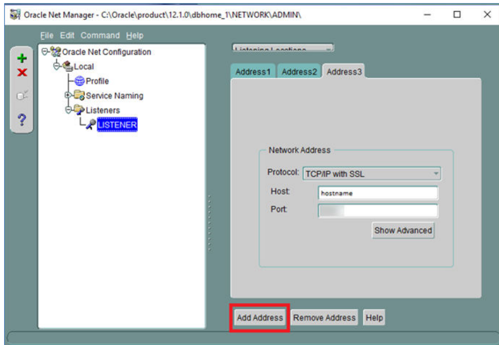
Figure 1-2 Listener, Address Tab
