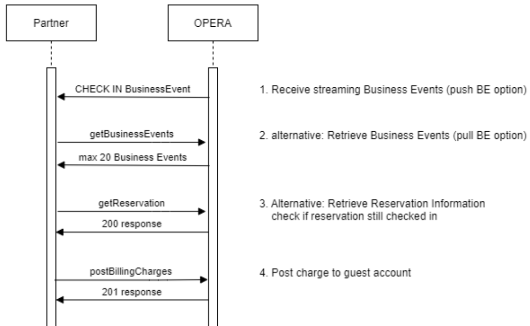
Figure 3-1 Sequence Diagram
