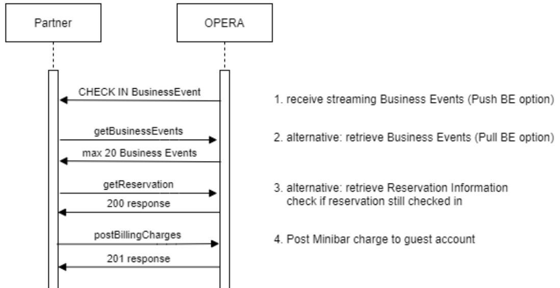
Figure 3-2 Sequence Diagram
