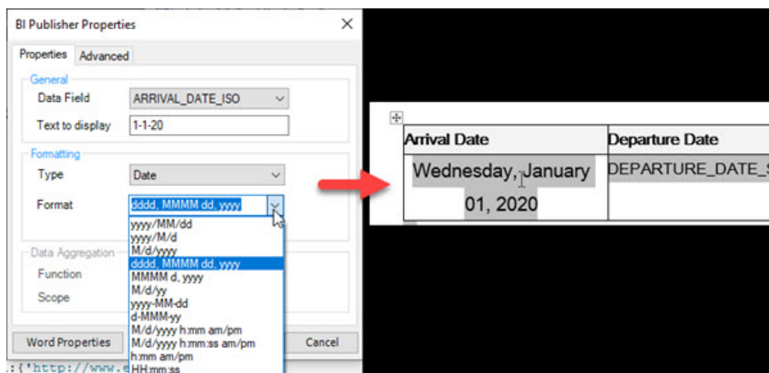
Figure 9-4 Formatting Dates
