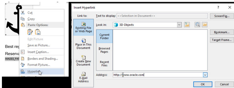
Figure 9-9 Insert Hyperlink
