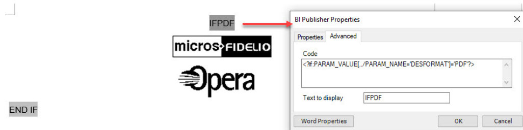
Figure 9-8 Conditional Image for PDF Output
