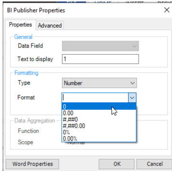
Figure 9-5 Formatting Numbers
