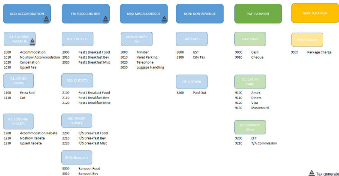
Figure 13-5 Transaction Codes
