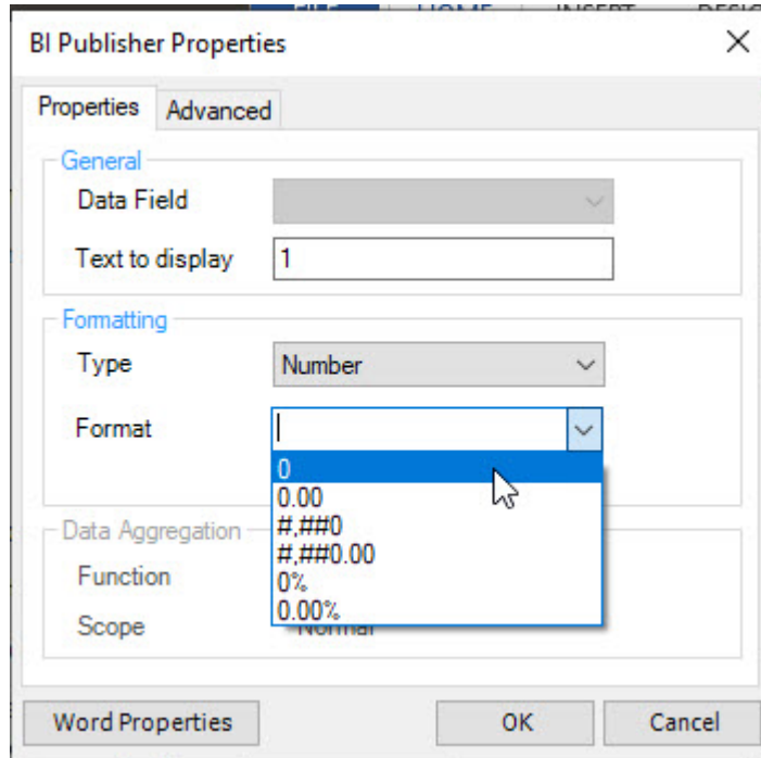
Figure 9-5 Formatting Numbers
