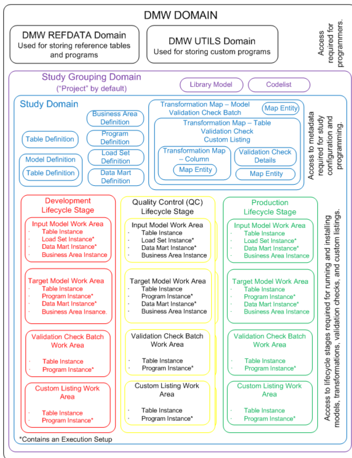
Figure 7-1 Object ownership
