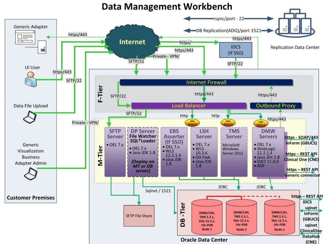
Figure 11-1 Oracle Life Sciences Data Management Workbench Architecture
