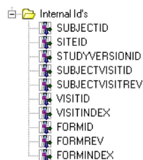
Figure 3-2 Cognos model
