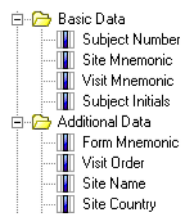
Figure 3-4 Cognos model
