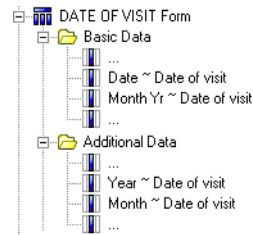
Figure 3-41 Cognos model
