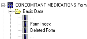
Figure 3-10 Cognos model
