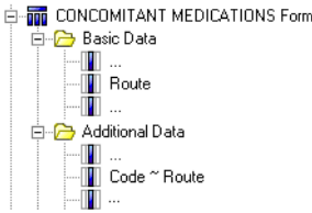
Figure 3-36 Cognos model
