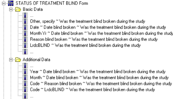
Figure 3-46 Cognos model
