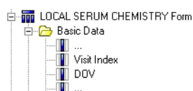
Figure 3-6 Cognos model
