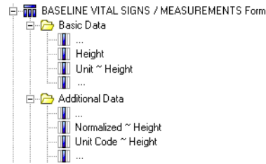
Figure 3-31 Cognos model
