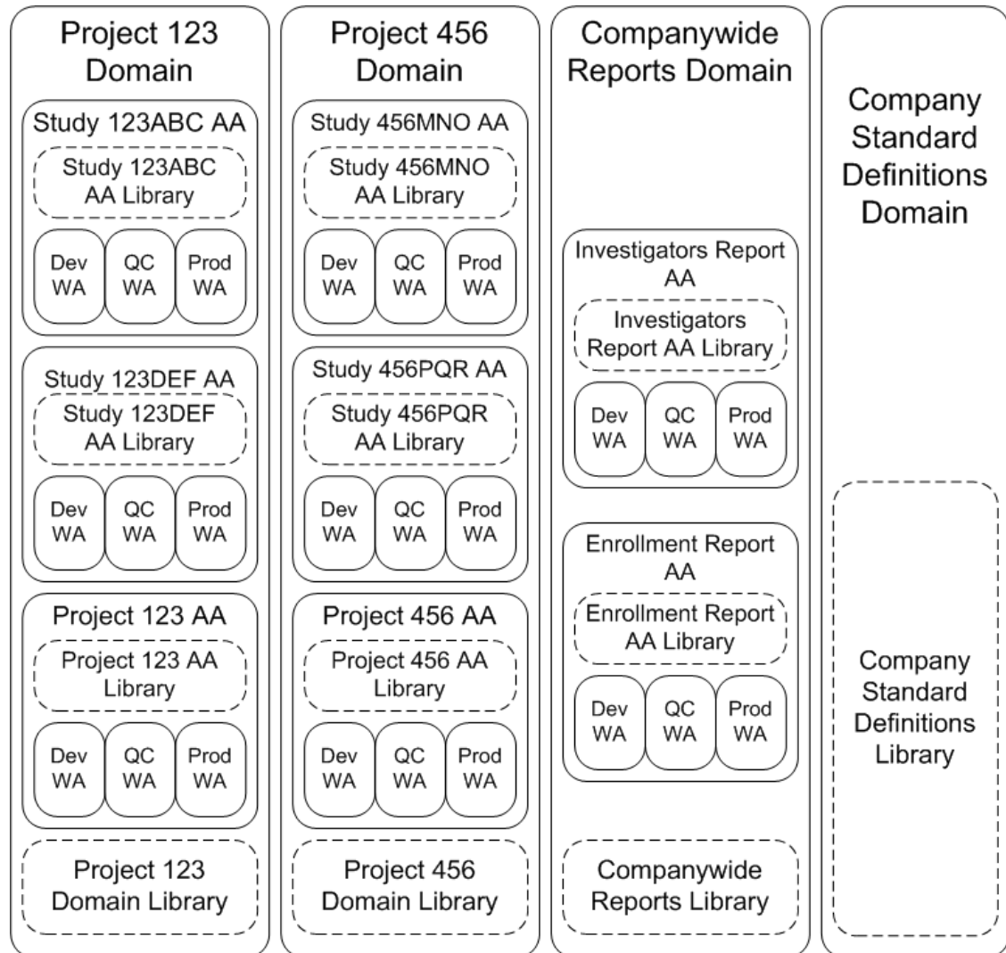
Figure 5-3 Example Organizational Structure
