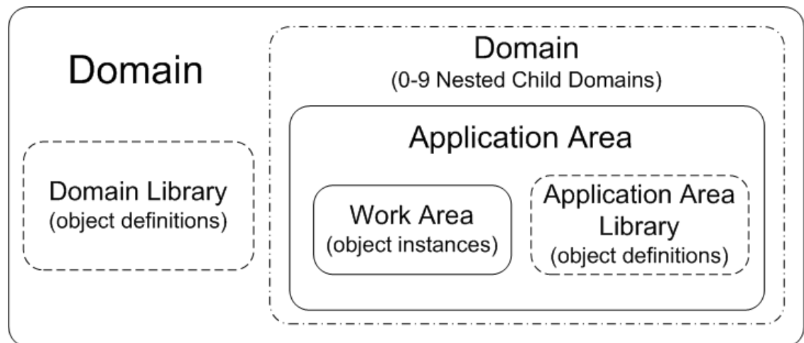
Figure 3-1 Oracle LSH Organizational Structure
