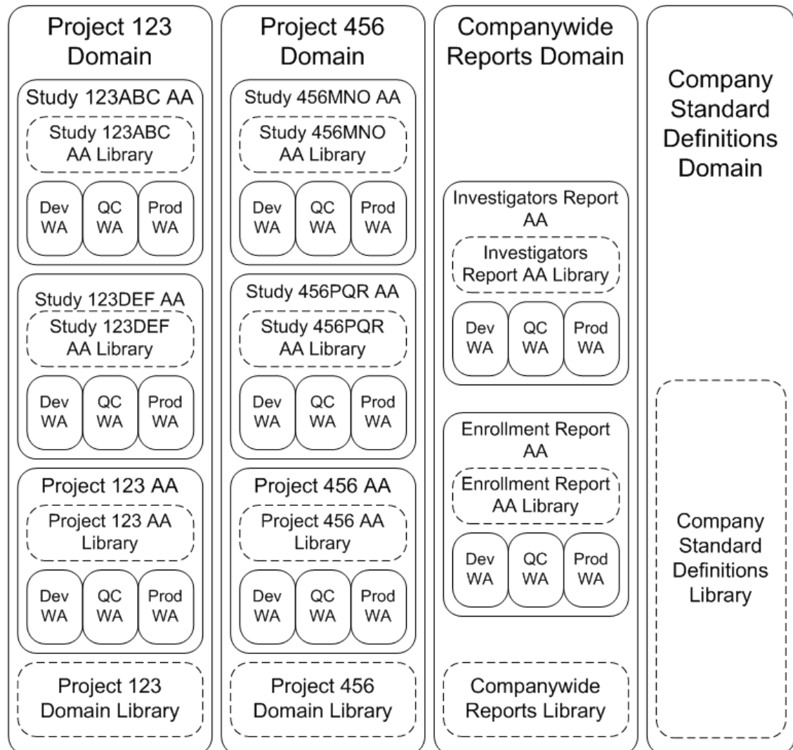
Figure 4-4 Organizational Structure for Security Design Example
