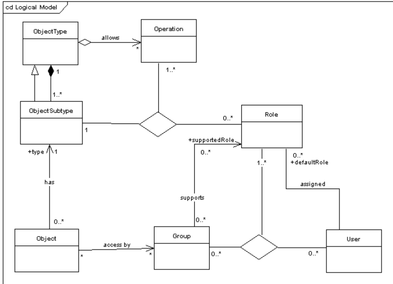
Figure 4-1 Logical Representation of the Object Security Elements and Their Relations
