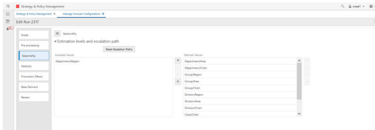
Figure 11-14 Edit Run
