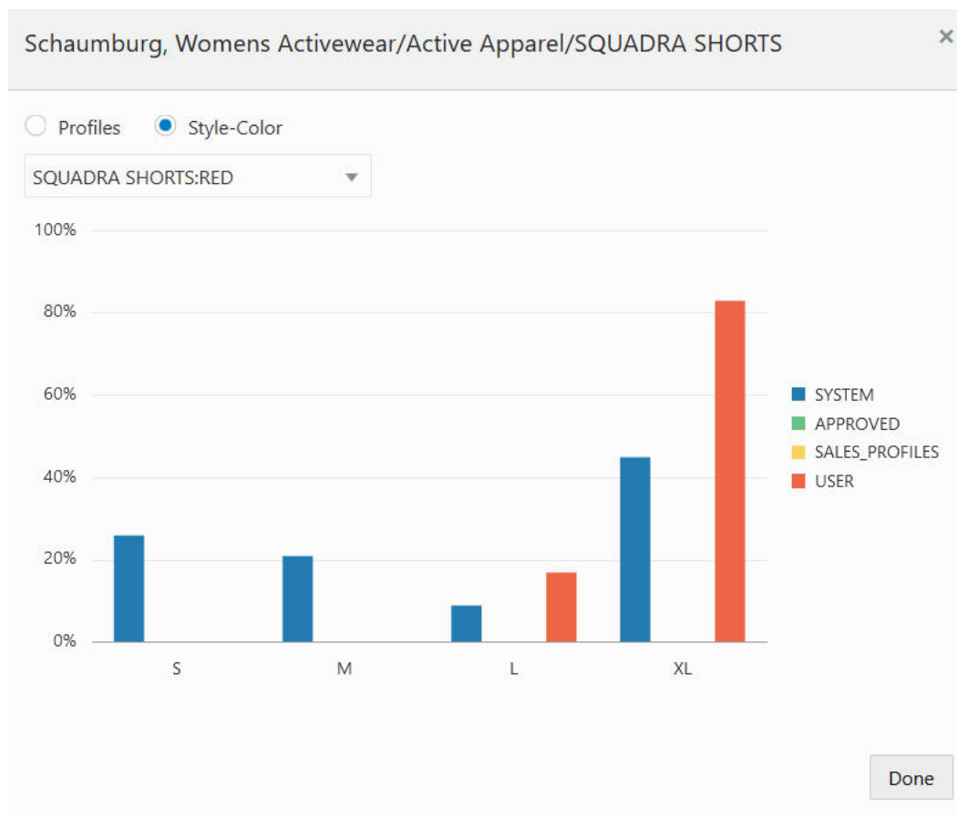
Figure 8-10 Colors View
