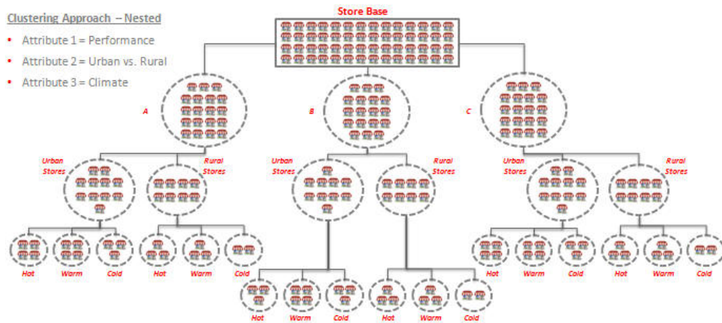
Figure 4-44 Nested Hierarchies
