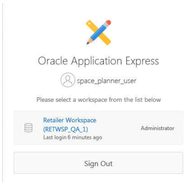
Figure 19-28 Retailer Workspace
