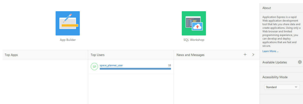
Figure 19-29 SQL Workspace
