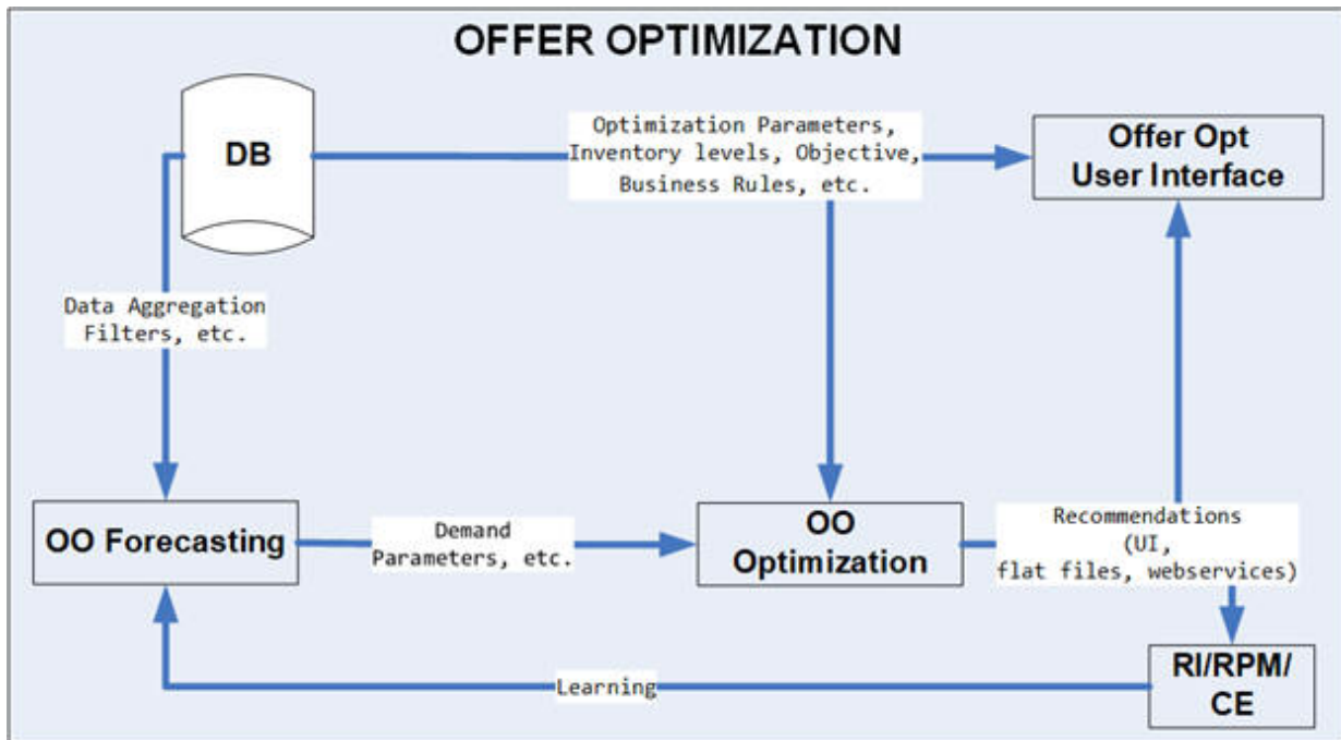
Figure 12-1 Offer Optimization
