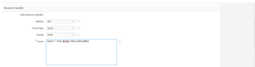
Figure 19-25 Resource Handler
