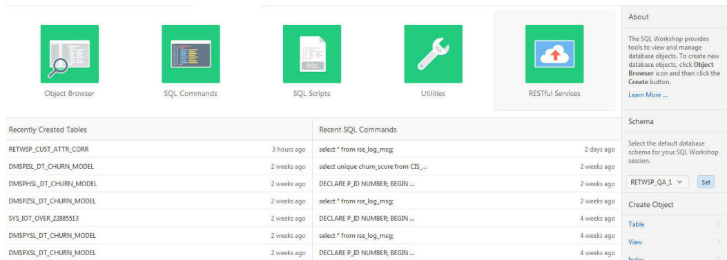
Figure 19-21 RESTful Service
