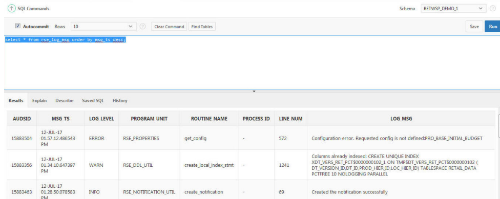
Figure 19-30 SQL Command
