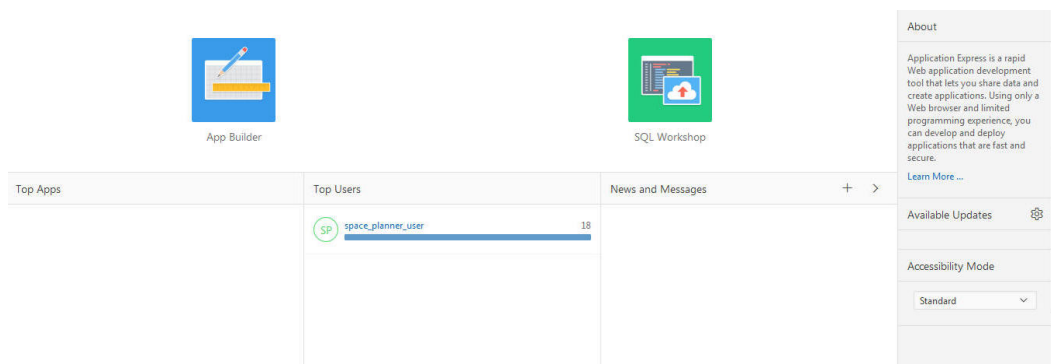
Figure 19-29 SQL Workspace
