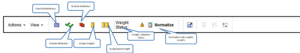
Figure 4-17 Attribute Toolbar
