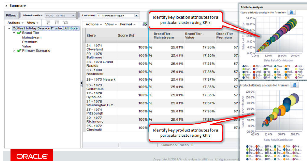
Figure 4-39 Attribute Analysis
