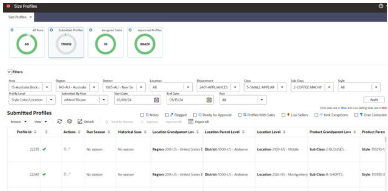
Figure 8-10 Submitted Profiles
