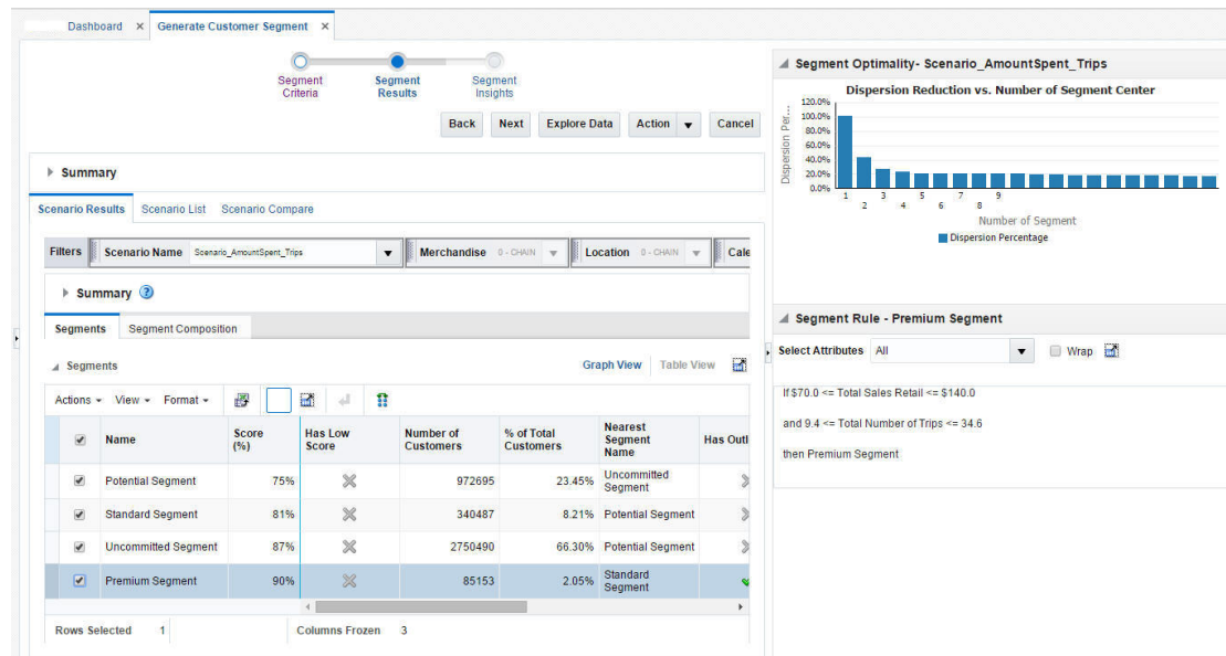
Figure 5-30 Segment Rules
