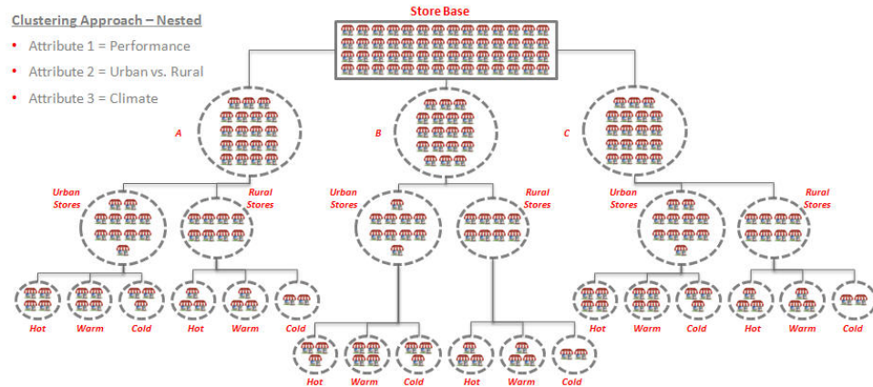
Figure 4-45 Nested Clusters
