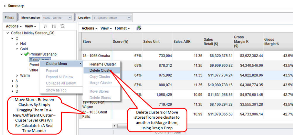
Figure 4-42 Delete Cluster
