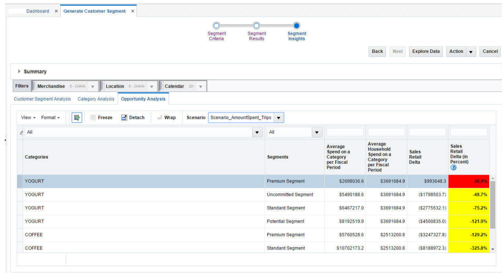
Figure 5-33 Opportunity Analysis
