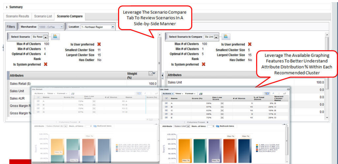
Figure 4-29 Compare Scenarios
