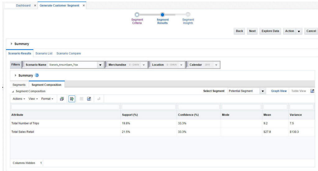
Figure 5-25 Segment Composition
