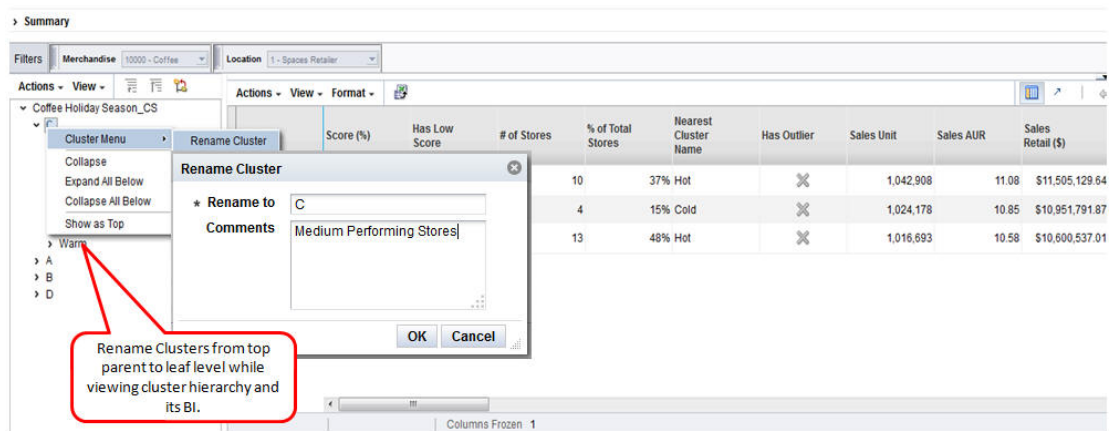
Figure 4-40 Rename Cluster
