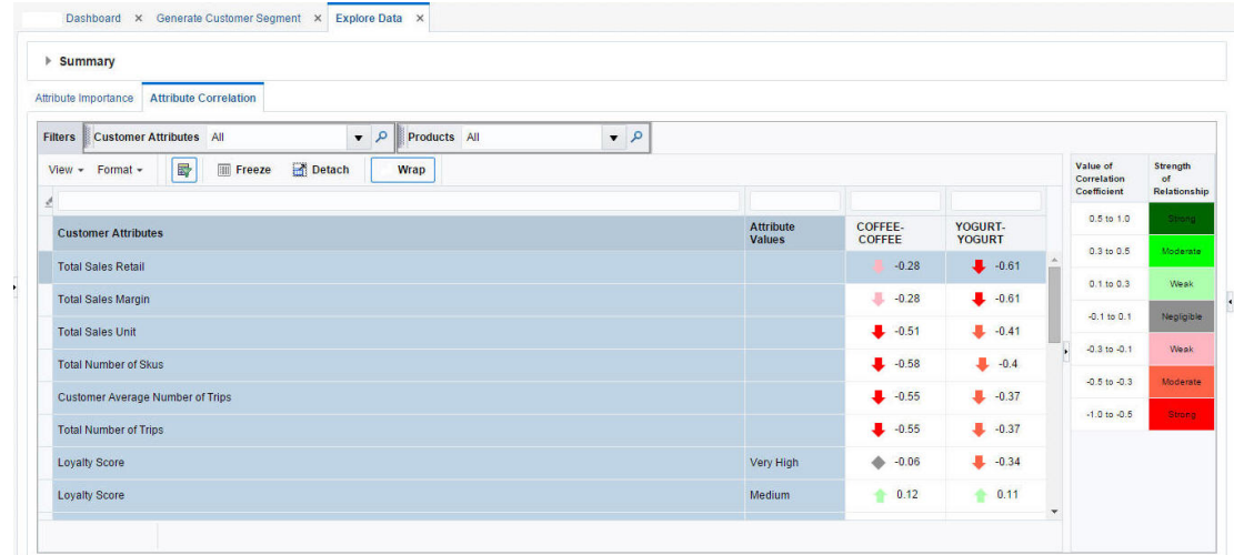
Figure 5-12 Attribute Correlation
