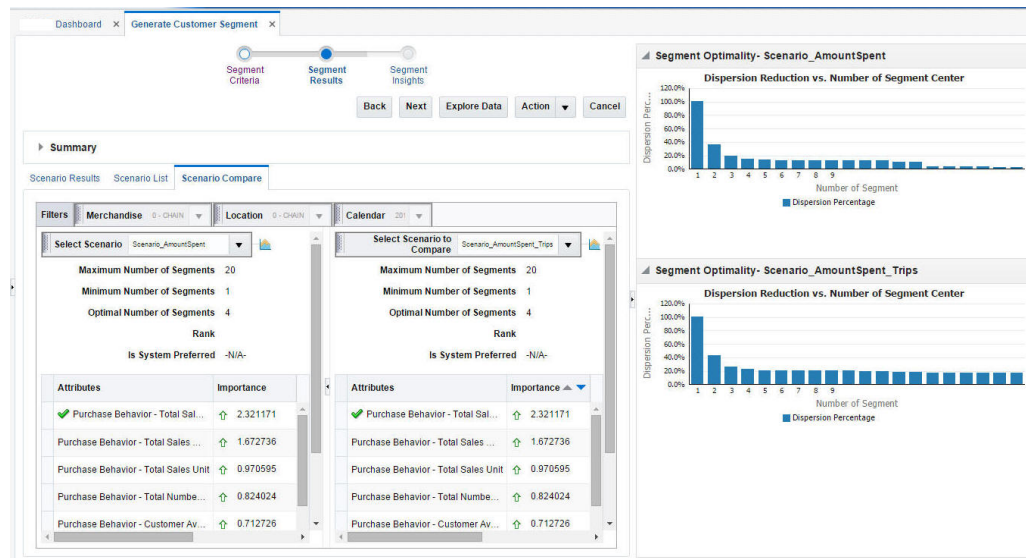
Figure 5-29 Scenario Optimality
