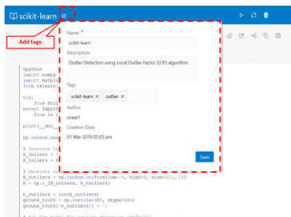
Figure 9-13 Notebook Tags
