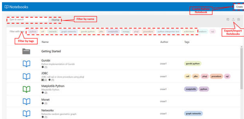
Figure 9-11 Notebook Functionality
