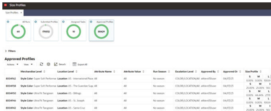
Figure 8-13 Approved Profiles
