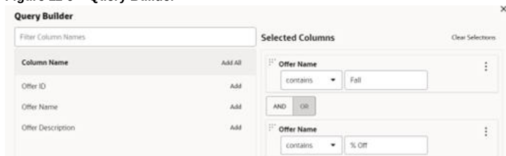
Figure 11-9 Query Builder
