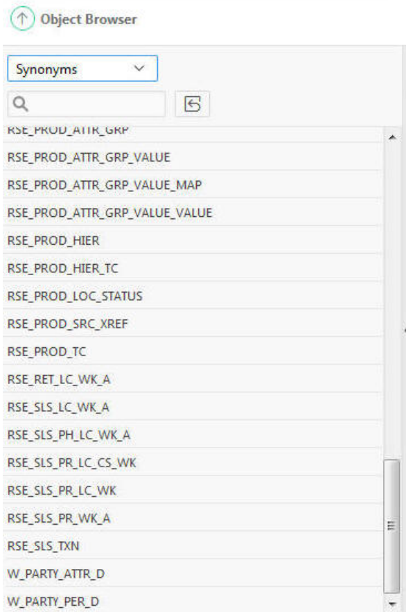
Figure 9-5 Contextual Area
