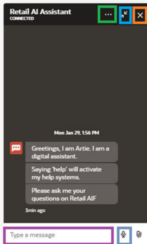
Figure 10-3 Chat Widget
