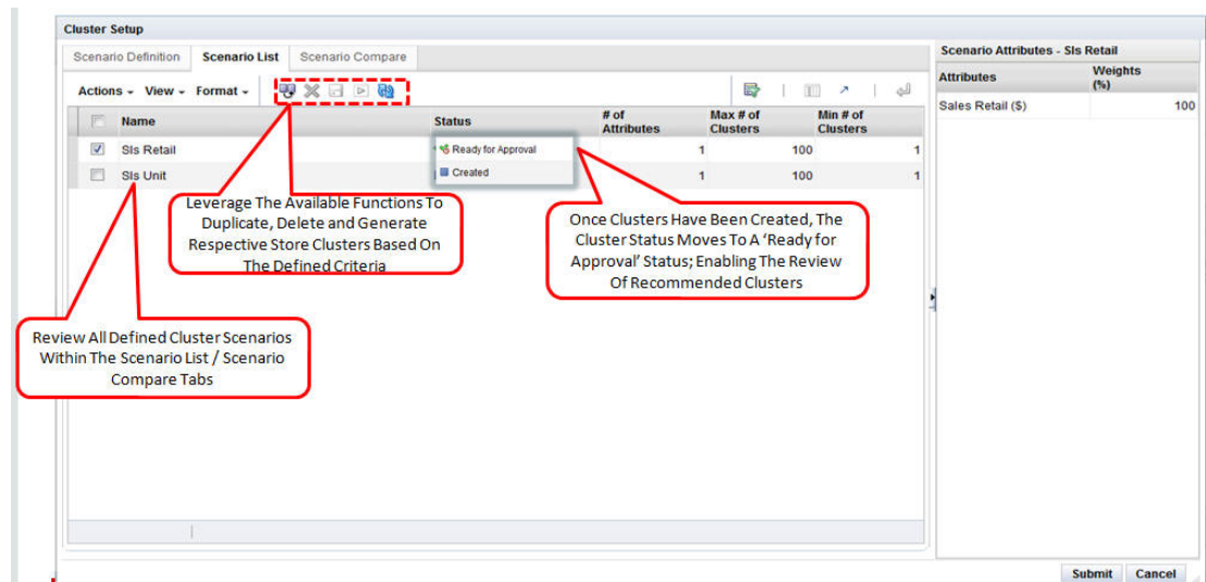
Figure 4-19 Scenario List
