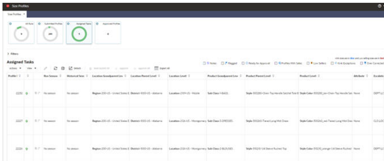
Figure 8-12 Assigned Tasks
