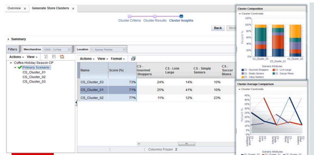
Figure 4-37 Cluster Comparison
