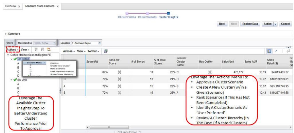
Figure 4-31 Clustering Insights
