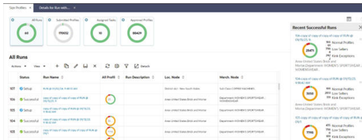
Figure 8-2 All Runs
