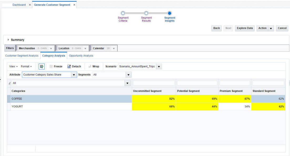
Figure 5-32 Category Analysis
