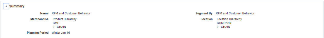
Figure 5-34 Summary
