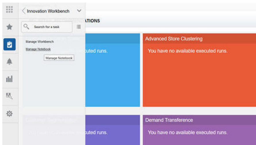
Figure 9-10 Manage Notebook
