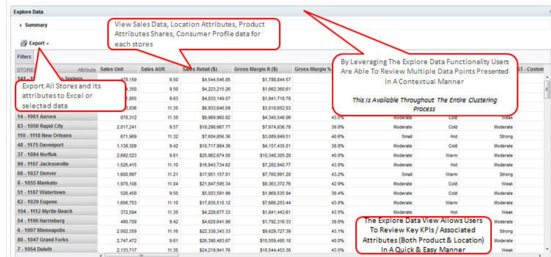
Figure 4-11 Explore Data
