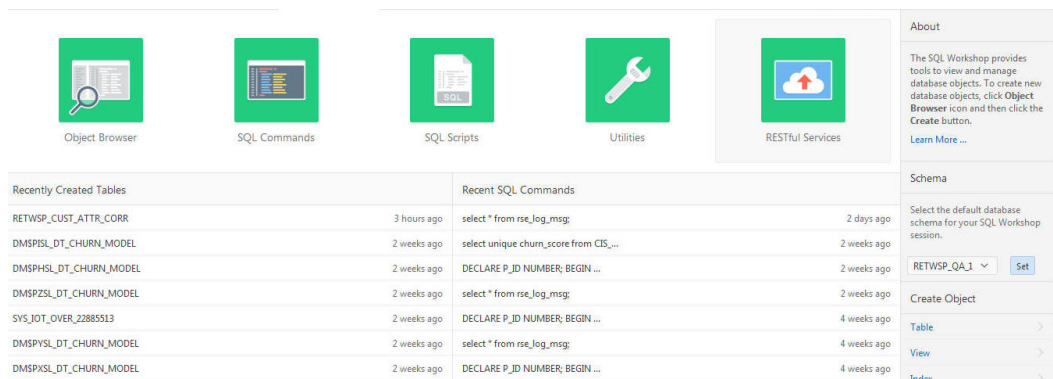
Figure 20-21 RESTful Service
