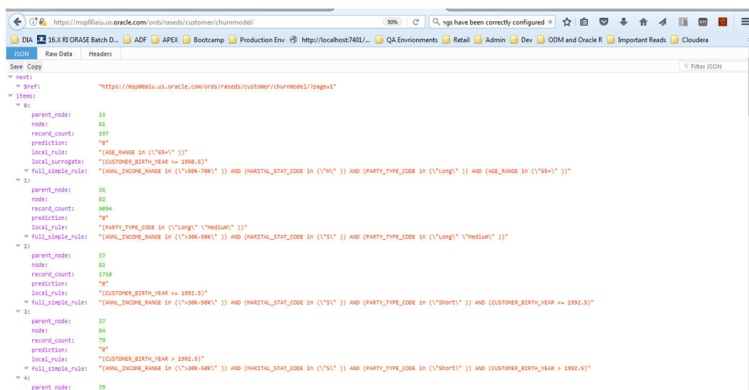
Figure 20-27 RESTful Refresh
