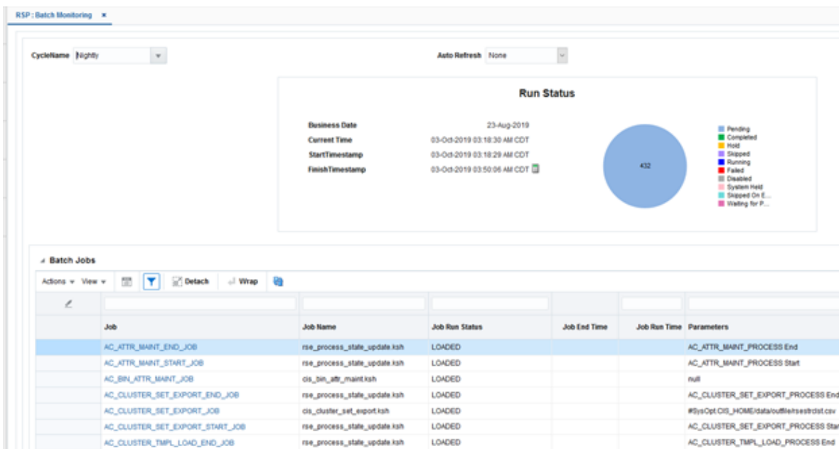
Figure 21-2 Batch Monitoring
