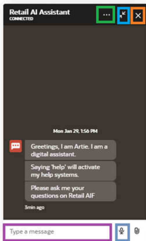
Figure 22-3 Chat Widget
