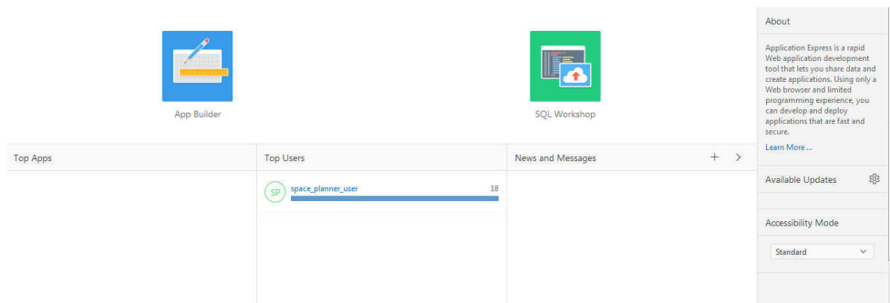
Figure 20-29 SQL Workspace
