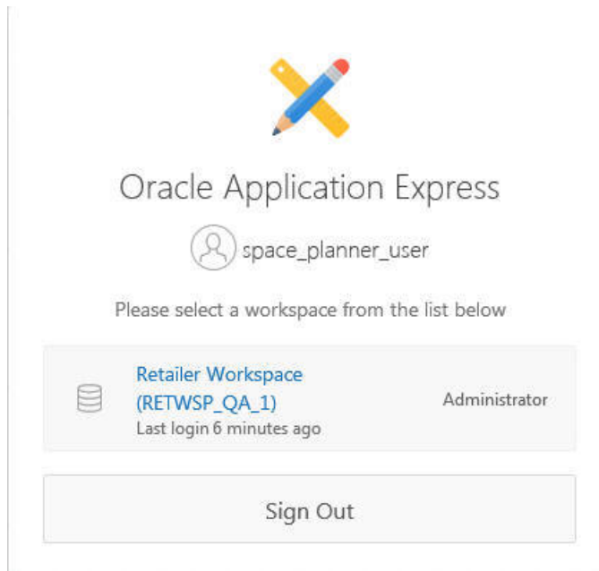
Figure 20-28 Retailer Workspace
