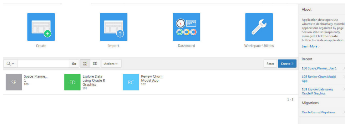
Figure 20-10 Application Builder
