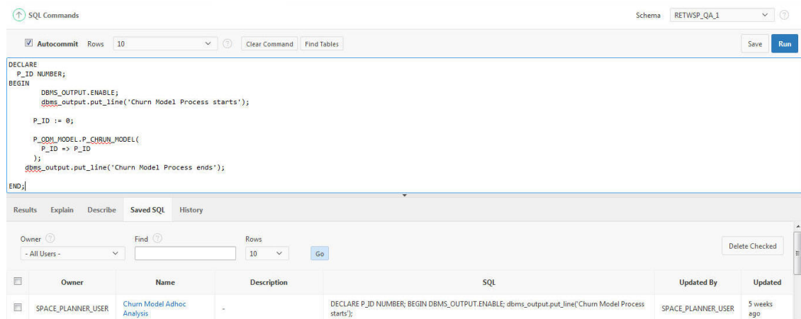
Figure 9-6 SQL Commands
