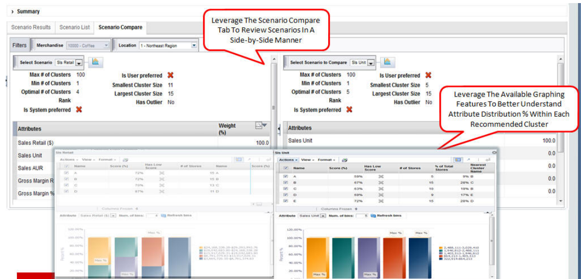
Figure 4-29 Compare Scenarios
