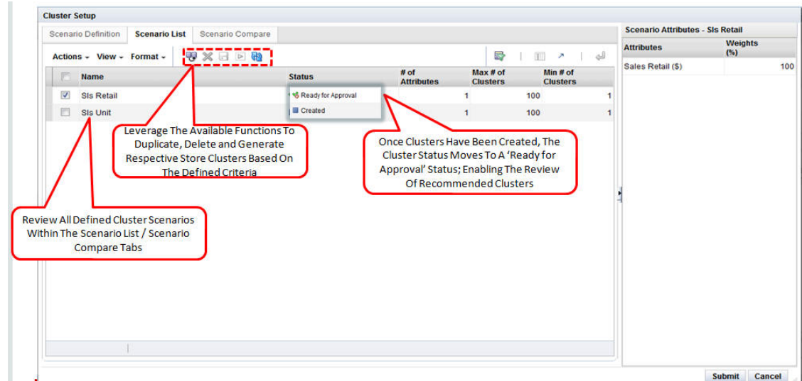
Figure 4-19 Scenario List
