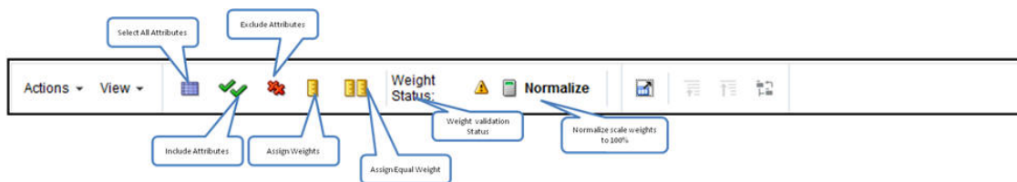
Figure 4-17 Attribute Toolbar
