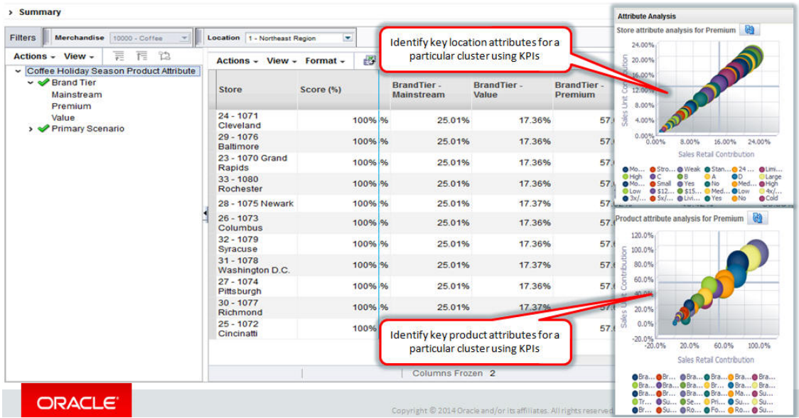
Figure 4-39 Attribute Analysis
