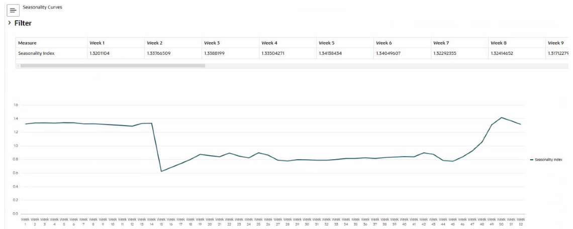
Figure 11-19 Seasonality
