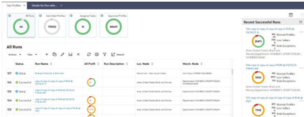
Figure 8-2 All Runs
