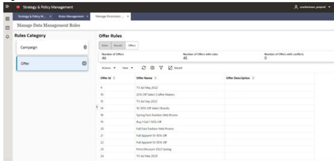
Figure 11-7 Offers
