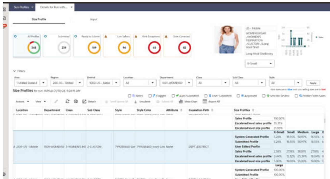
Figure 8-7 Run Output
