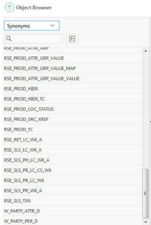
Figure 9-5 Contextual Area
