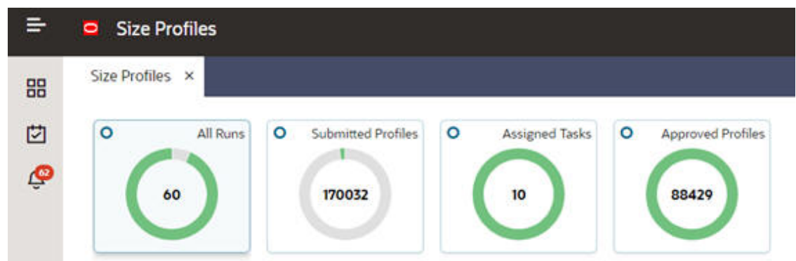
Figure 8-1 Info Tiles
