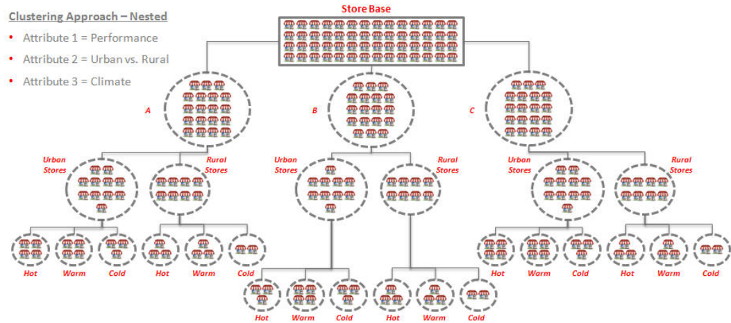
Figure 4-45 Nested Clusters
