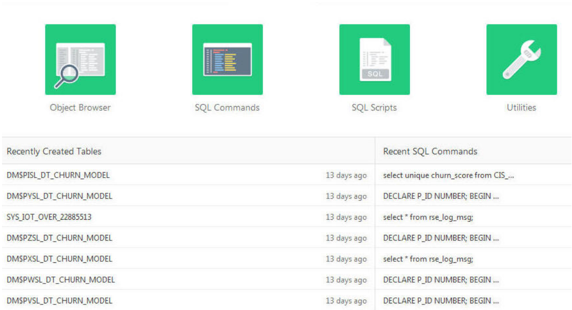
Figure 9-4 SQL Workshop
