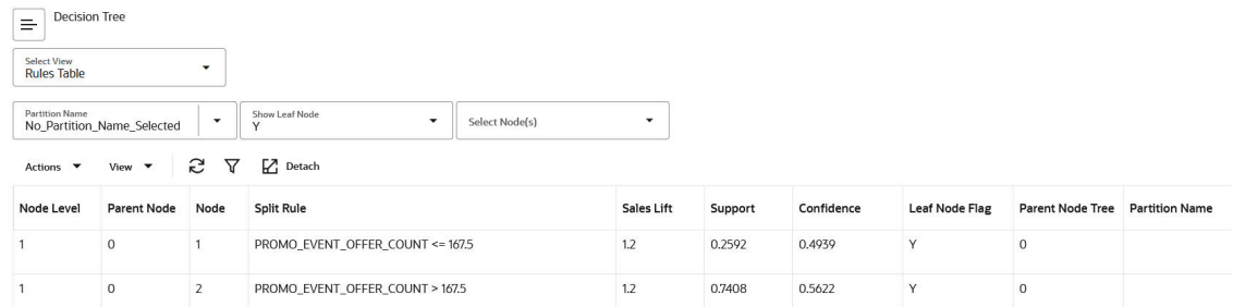
Figure 11-20 Decision Tree
