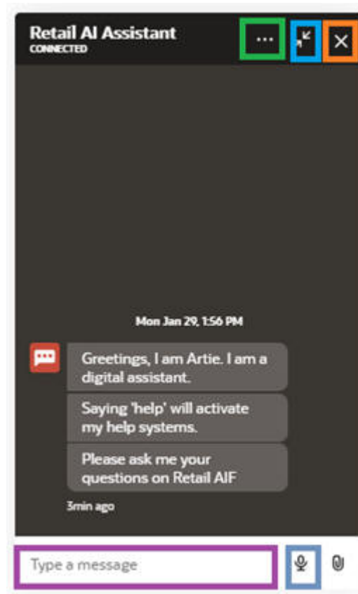
Figure 10-3 Chat Widget
