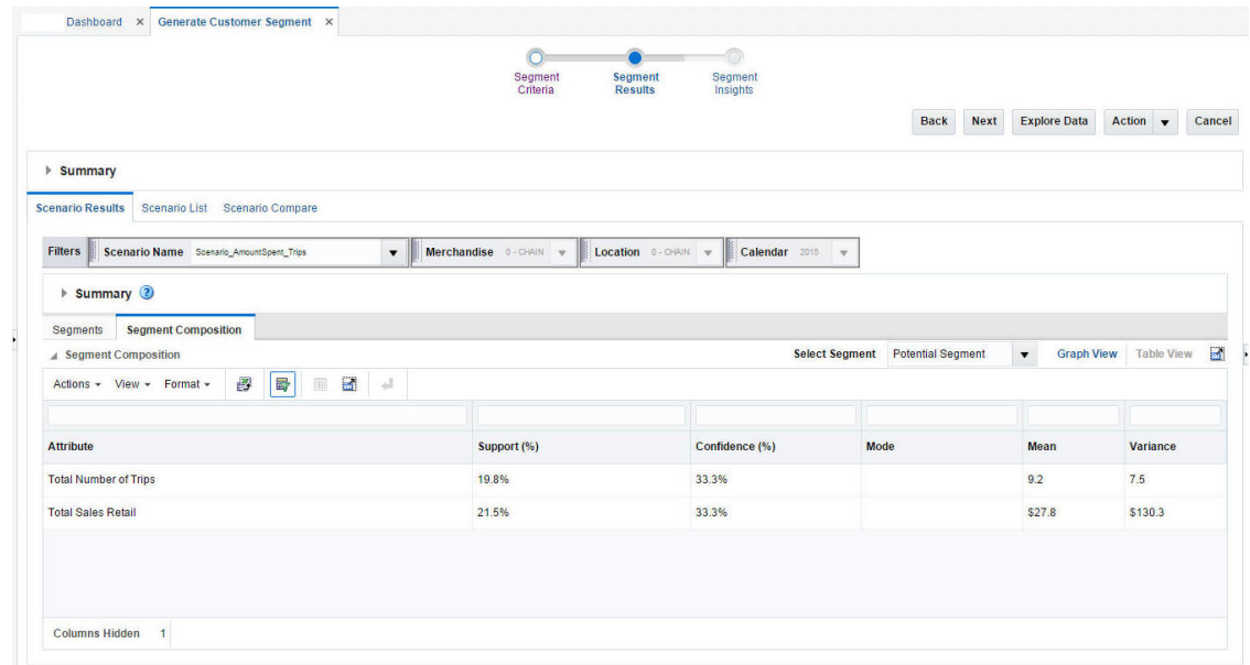
Figure 5-25 Segment Composition
