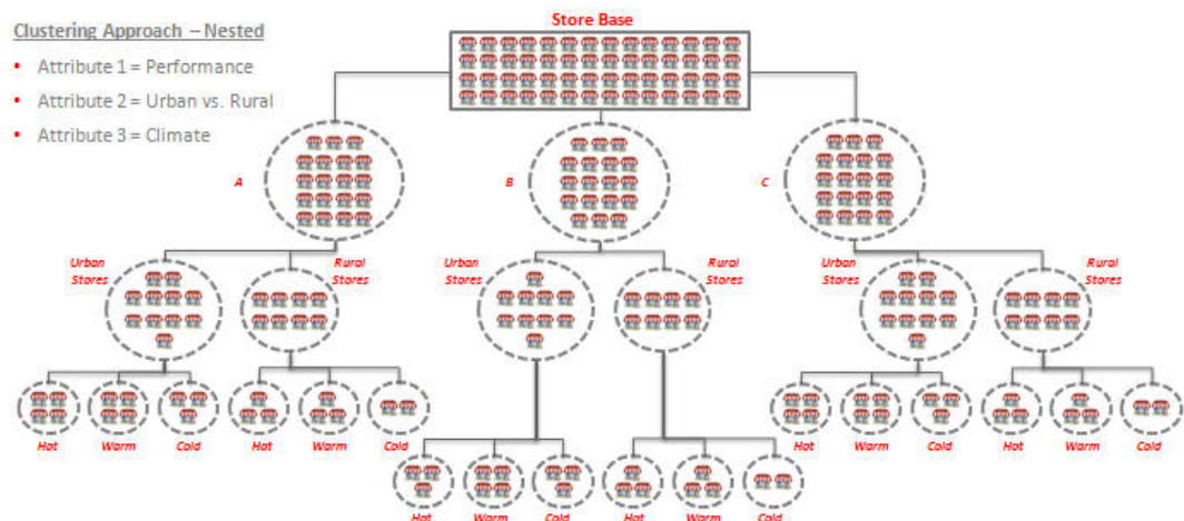
Figure 4-44 Nested Hierarchies
