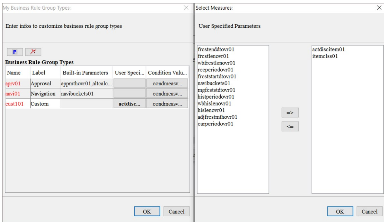
Figure 3-8 Select User Specified Parameters
