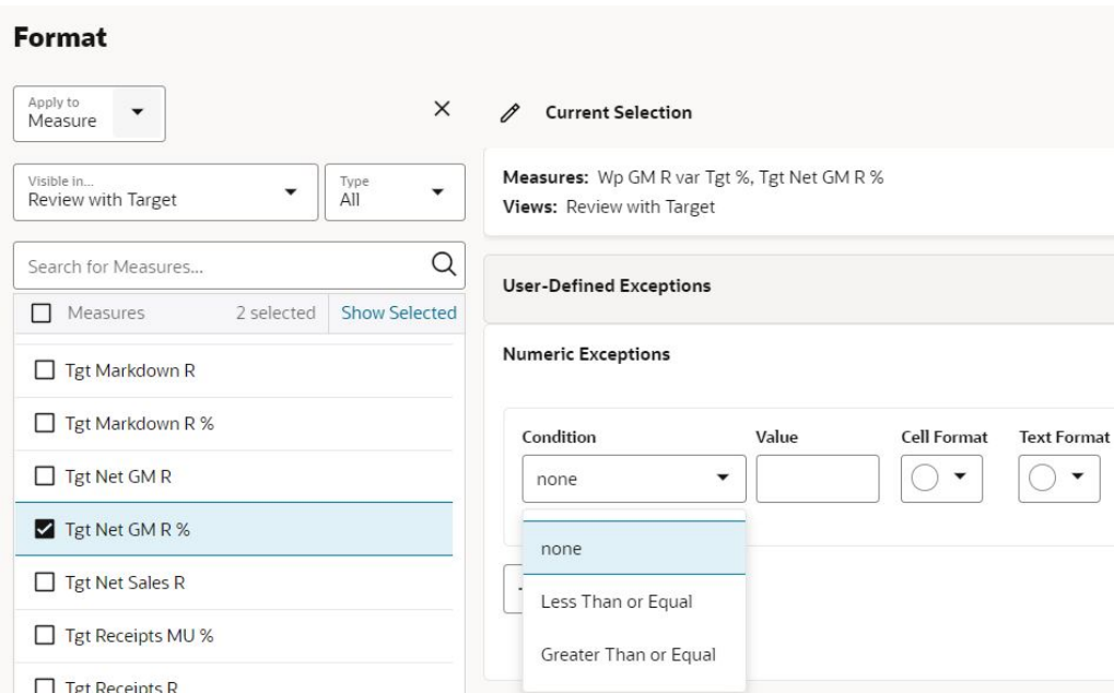
Figure 9-17 Format Dialog
