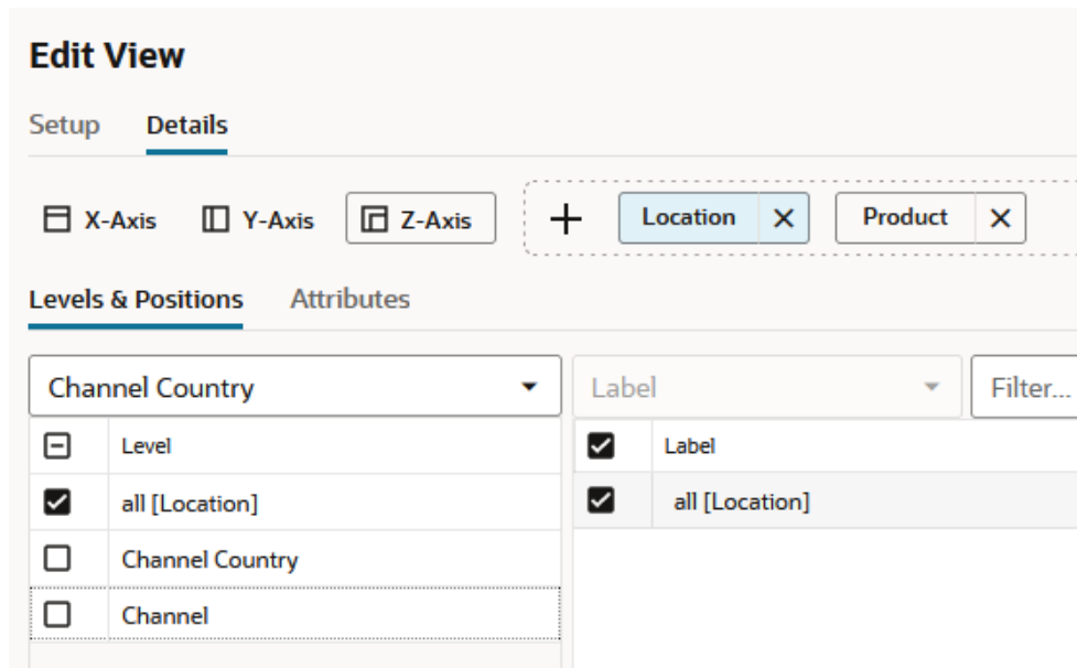
Figure 9-4 Location Dimension Selection Window
