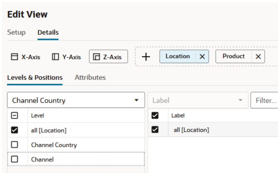
Figure 8-4 Location Dimension Selection Window
