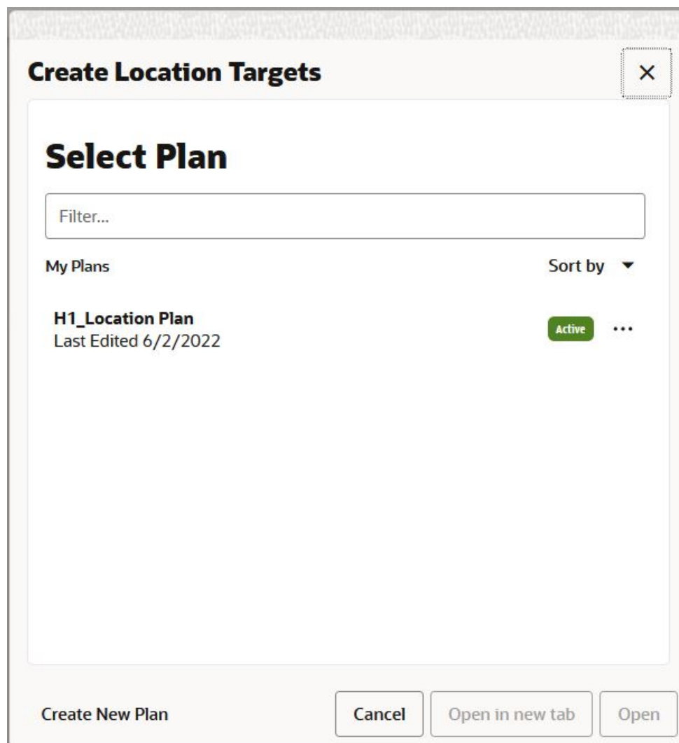
Figure 3-4 Create Dialog
