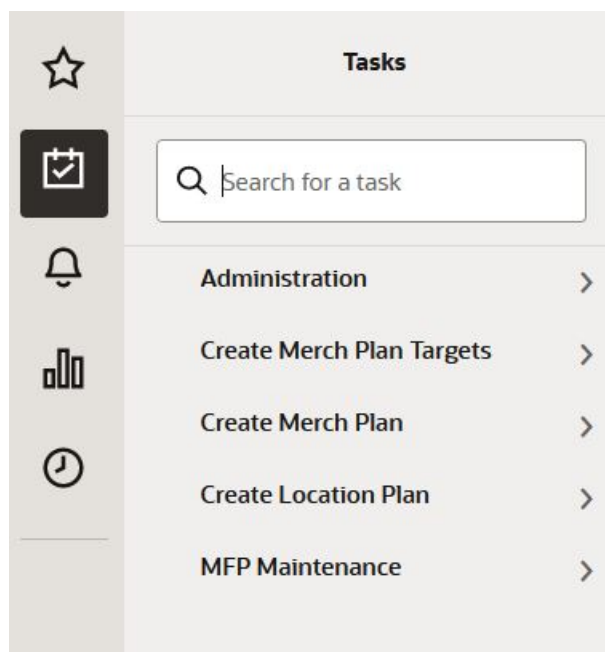
Figure 3-1 Tasks Menu
