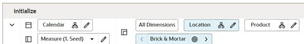
Figure 9-3 Location Tile
