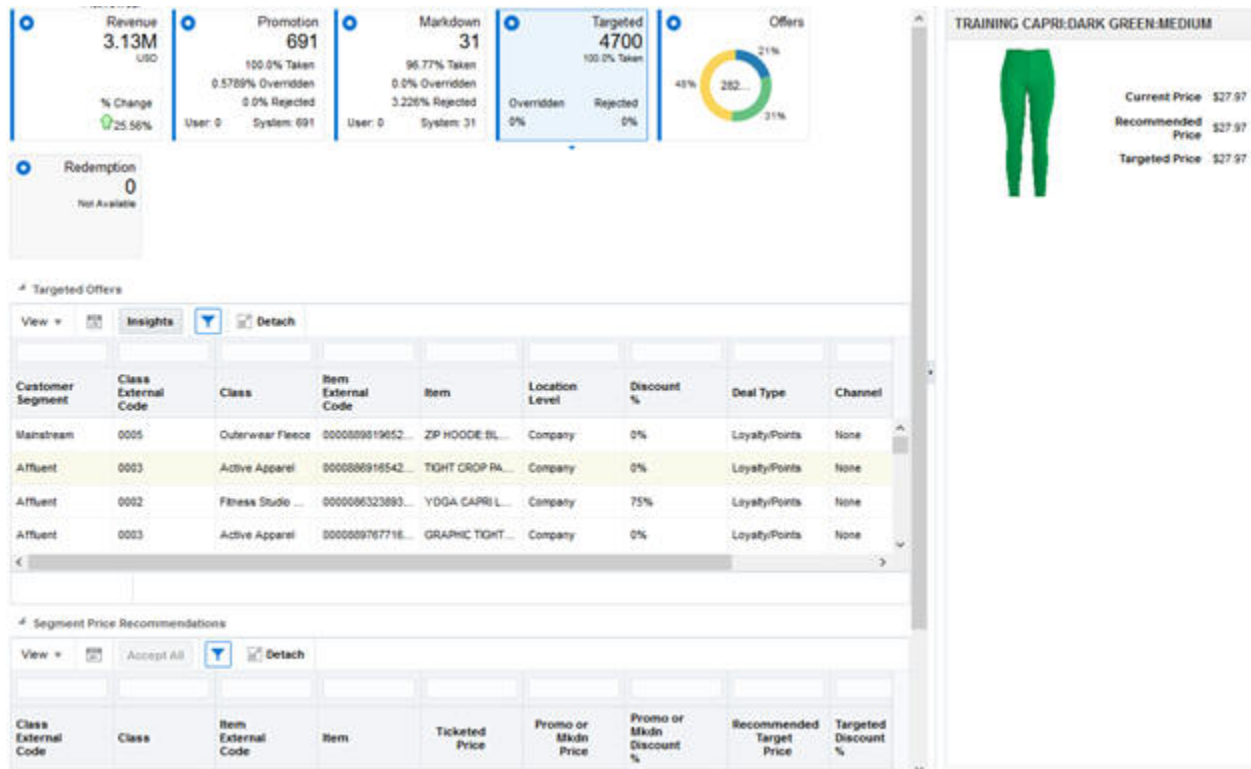
Figure 1-29 Targeted Tile
