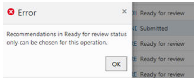
Figure 1-37 Accept
