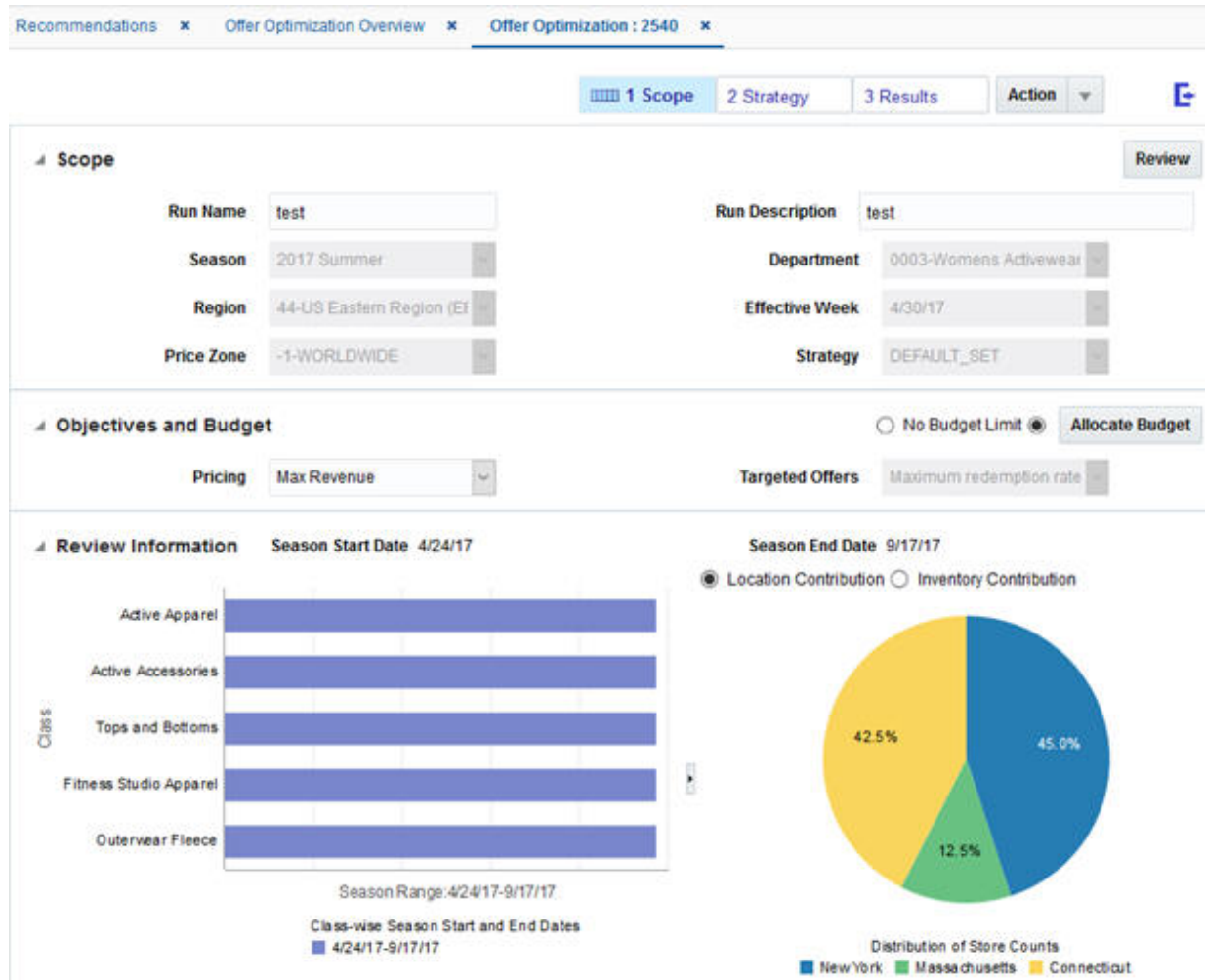
Figure 1-10 Setup
