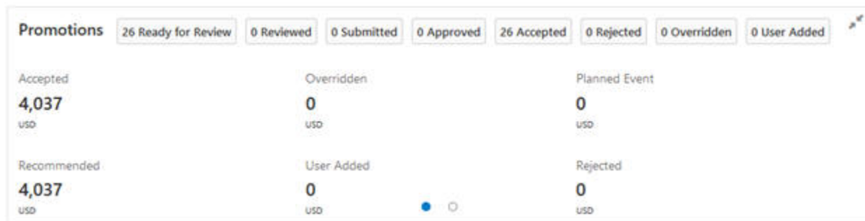
Figure 1-34 Summary Metrics
