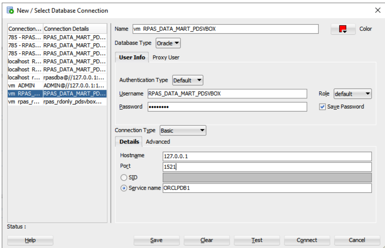
Figure 3-19 Database Connection
