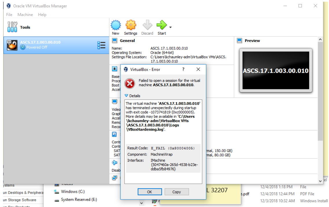
Figure 3-20 VirtualBox Error
