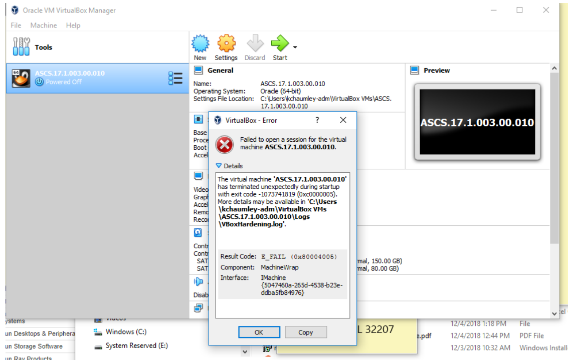
Figure 3-20 VirtualBox Error
