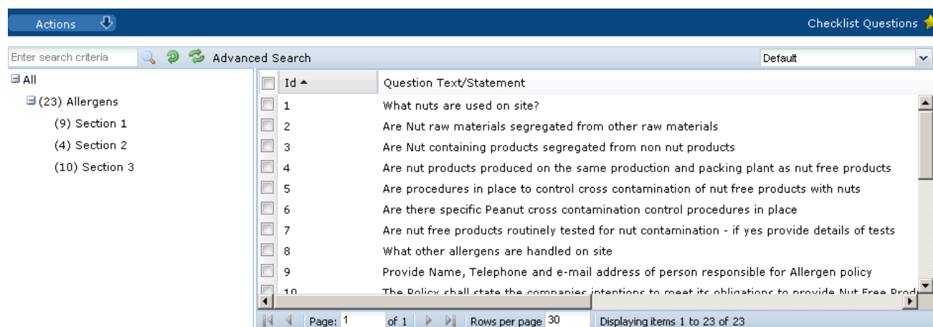
Figure 7-34 Checklist Questions
