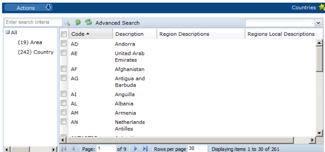
Figure 7-12 Countries Page
