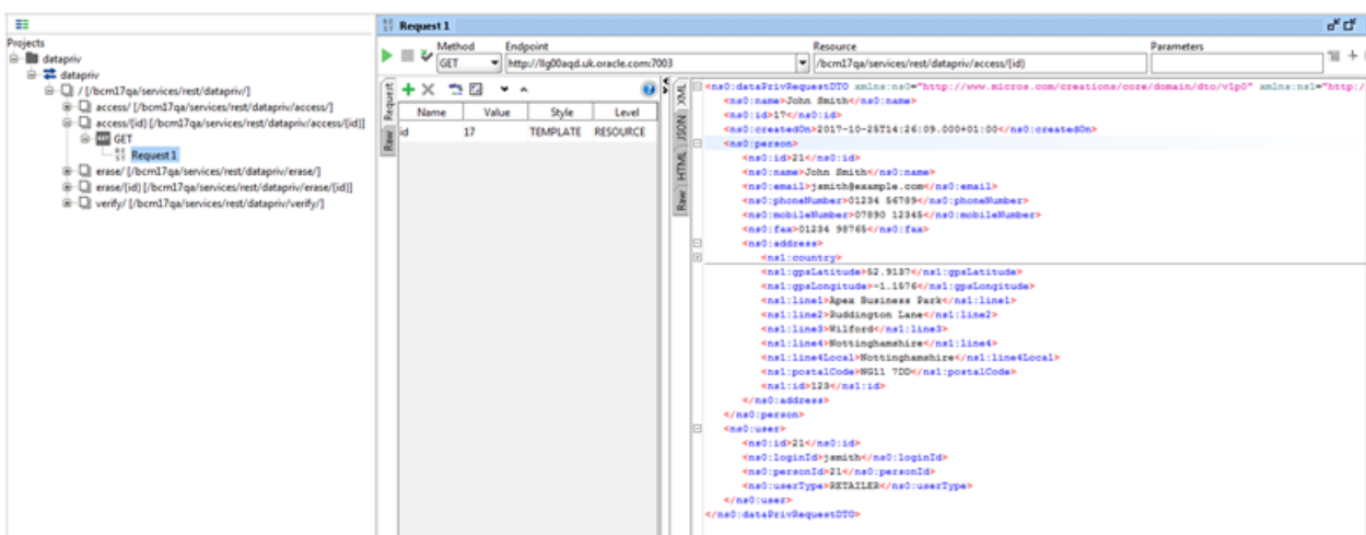
Figure B-3 Access Get Request
